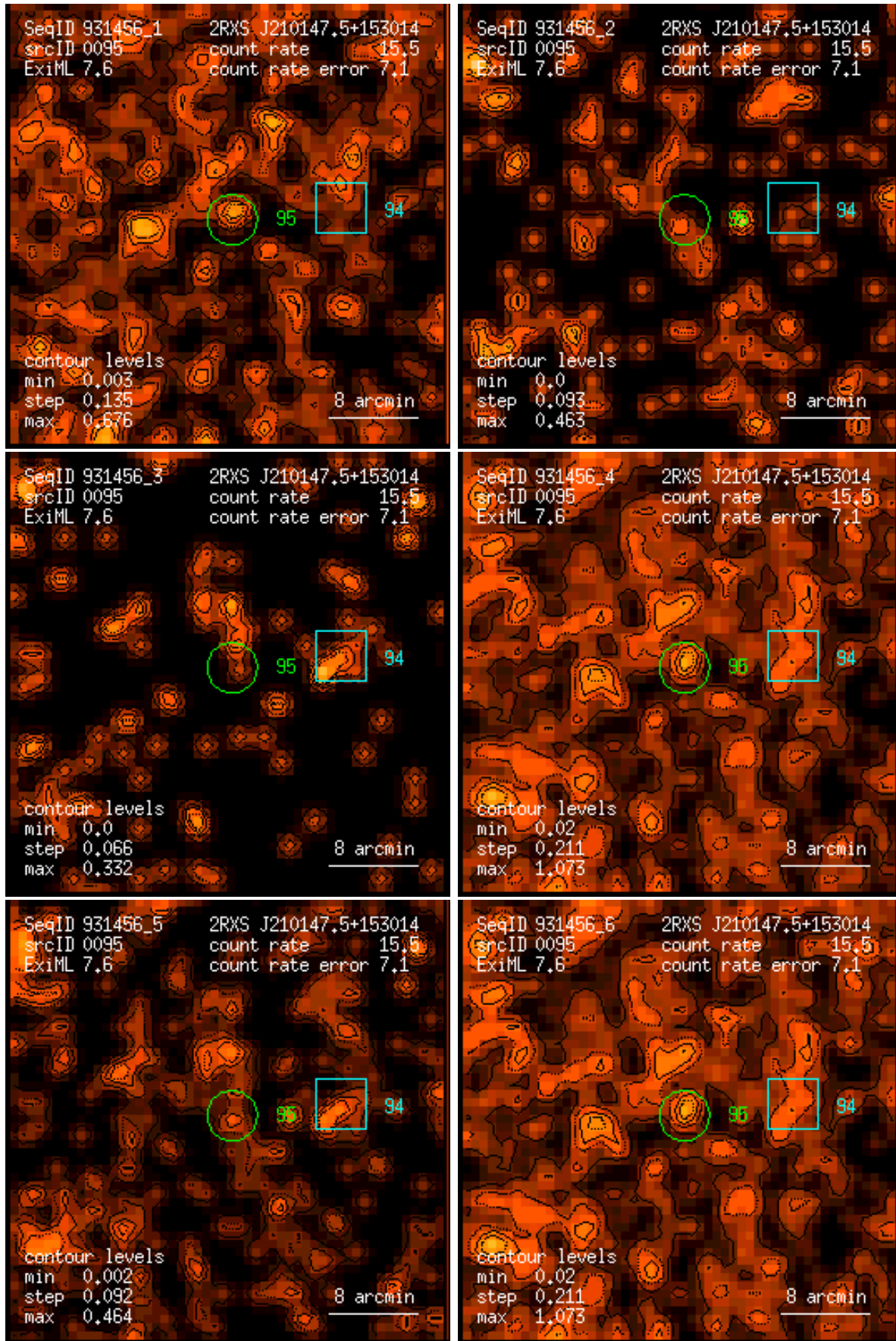
Figure 95: RASS 931456: detection 0095: band rate images, Gaussian filter: (1) PSPC channels 11 – 41, (2) 52 – 90, (3) 91 – 201, (4) 11 – 235, (5) 52 – 201, (6) 11 – 201. Broad band rates in counts/ks. Band rate contour levels in counts/ks/arcmin 2 .
