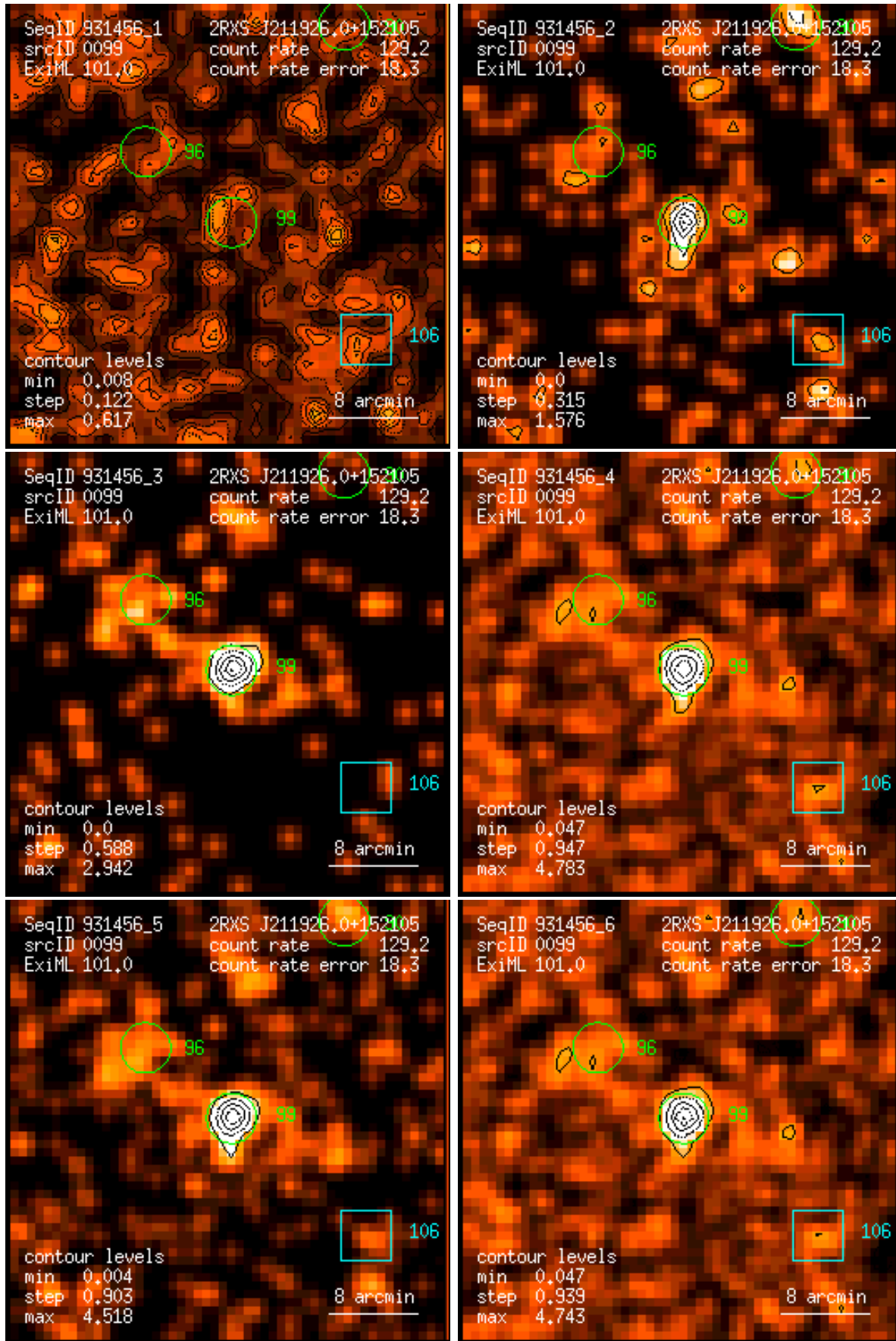
Figure 99: RASS 931456: detection 0099: band rate images, Gaussian filter: (1) PSPC channels 11 – 41, (2) 52 – 90, (3) 91 – 201, (4) 11 – 235, (5) 52 – 201, (6) 11 – 201. Broad band rates in counts/ks. Band rate contour levels in counts/ks/arcmin 2 .
