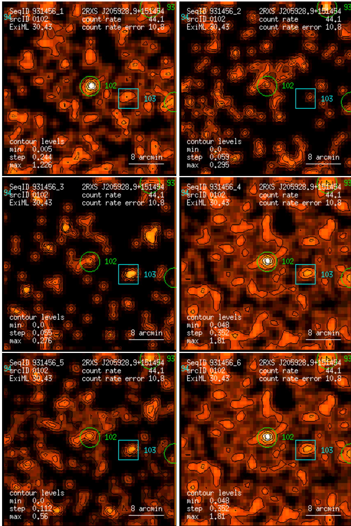
Figure 102: RASS 931456: detection 0102: band rate images, Gaussian filter: (1) PSPC channels 11 – 41, (2) 52 – 90, (3) 91 – 201, (4) 11 – 235, (5) 52 – 201, (6) 11 – 201. Broad band rates in counts/ks. Band rate contour levels in counts/ks/arcmin 2 .
