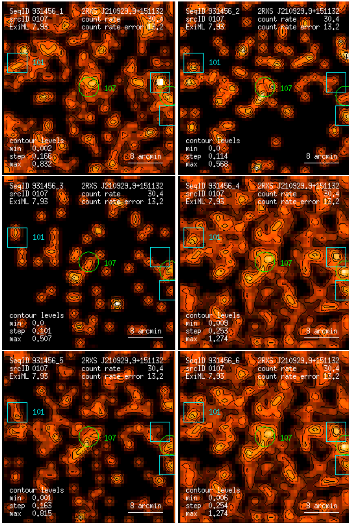
Figure 107: RASS 931456: detection 0107: band rate images, Gaussian filter: (1) PSPC channels 11 – 41, (2) 52 – 90, (3) 91 – 201, (4) 11 – 235, (5) 52 – 201, (6) 11 – 201. Broad band rates in counts/ks. Band rate contour levels in counts/ks/arcmin 2 .
