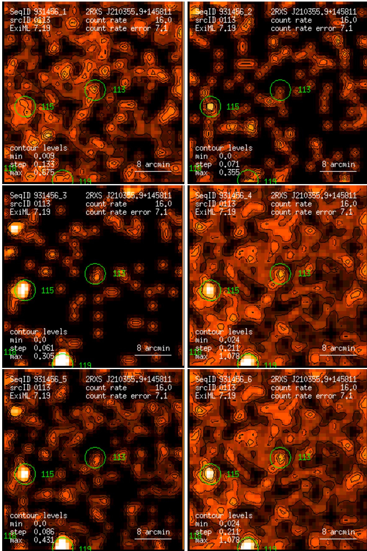
Figure 113: RASS 931456: detection 0113: band rate images, Gaussian filter: (1) PSPC channels 11 – 41, (2) 52 – 90, (3) 91 – 201, (4) 11 – 235, (5) 52 – 201, (6) 11 – 201. Broad band rates in counts/ks. Band rate contour levels in counts/ks/arcmin 2 .
