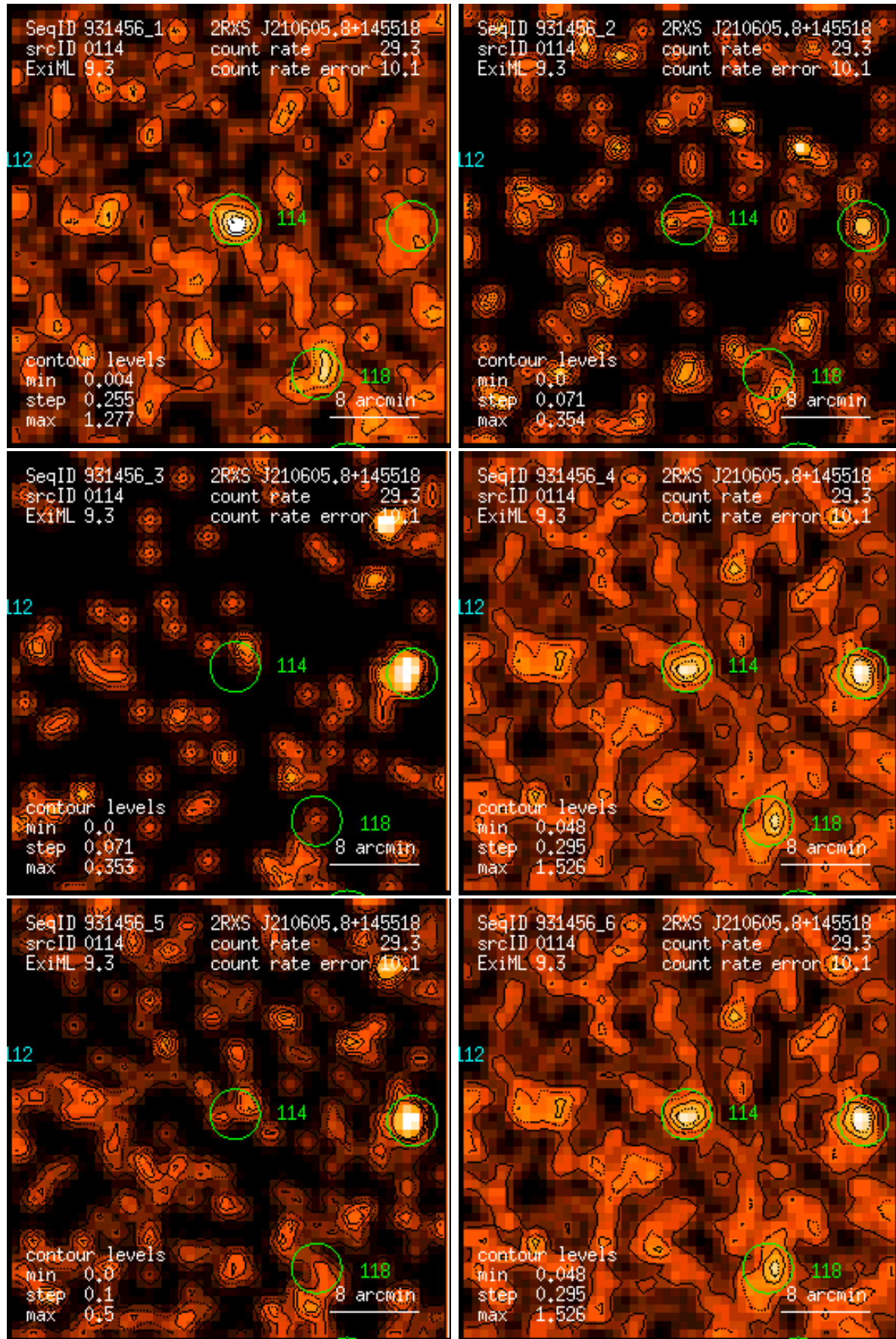
Figure 114: RASS 931456: detection 0114: band rate images, Gaussian filter: (1) PSPC channels 11 – 41, (2) 52 – 90, (3) 91 – 201, (4) 11 – 235, (5) 52 – 201, (6) 11 – 201. Broad band rates in counts/ks. Band rate contour levels in counts/ks/arcmin 2 .
