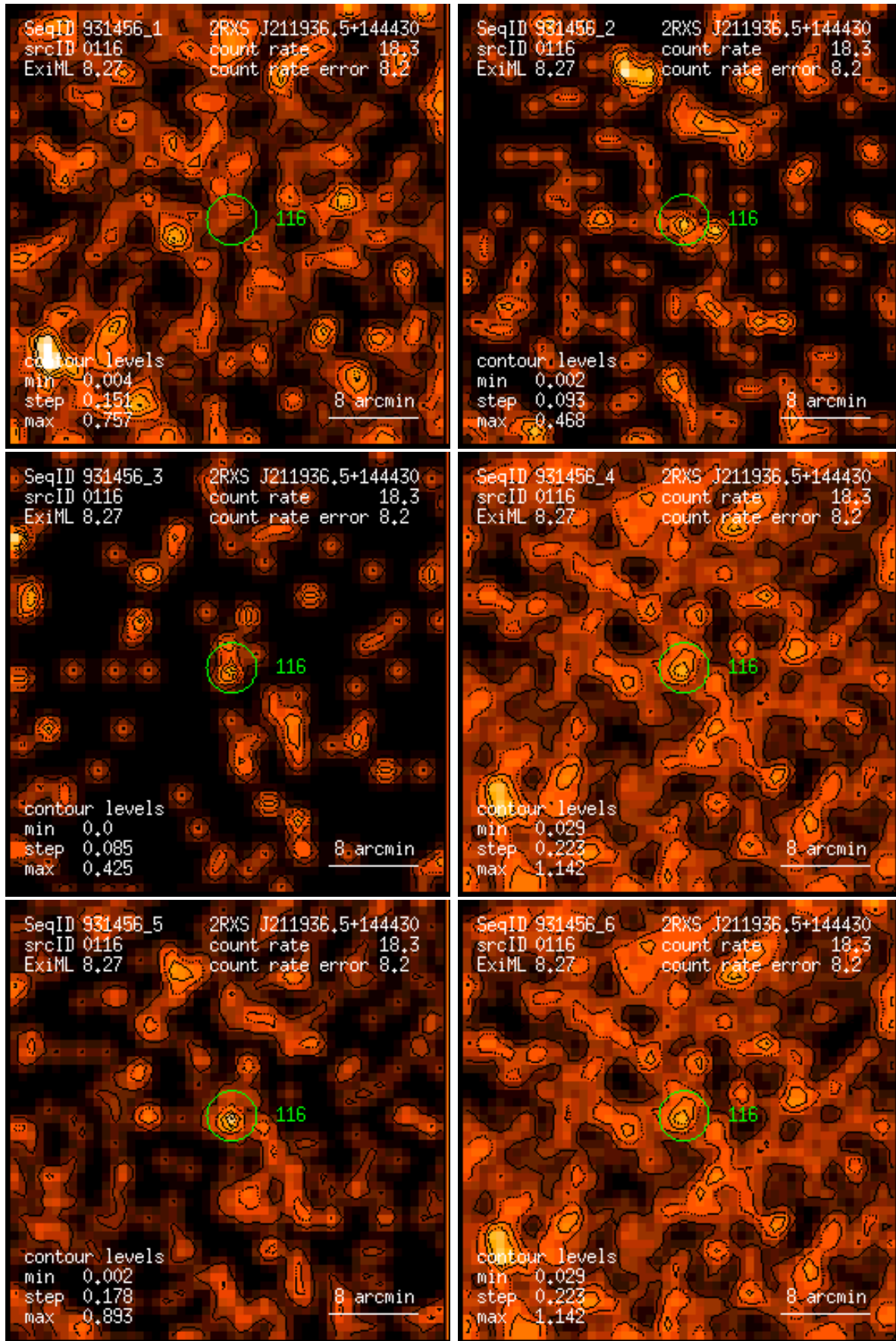
Figure 116: RASS 931456: detection 0116: band rate images, Gaussian filter: (1) PSPC channels 11 – 41, (2) 52 – 90, (3) 91 – 201, (4) 11 – 235, (5) 52 – 201, (6) 11 – 201. Broad band rates in counts/ks. Band rate contour levels in counts/ks/arcmin 2 .
