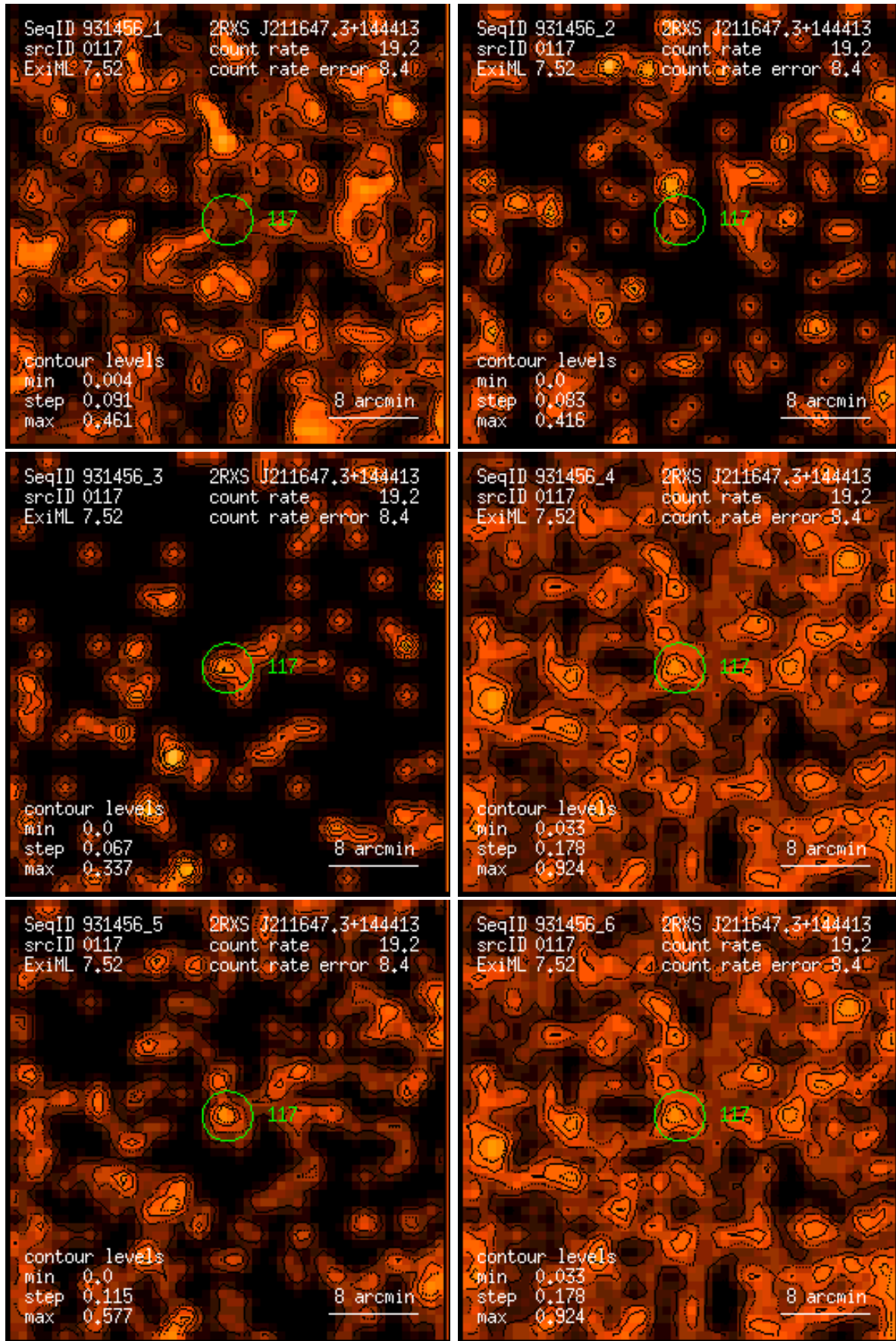
Figure 117: RASS 931456: detection 0117: band rate images, Gaussian filter: (1) PSPC channels 11 – 41, (2) 52 – 90, (3) 91 – 201, (4) 11 – 235, (5) 52 – 201, (6) 11 – 201. Broad band rates in counts/ks. Band rate contour levels in counts/ks/arcmin 2 .
