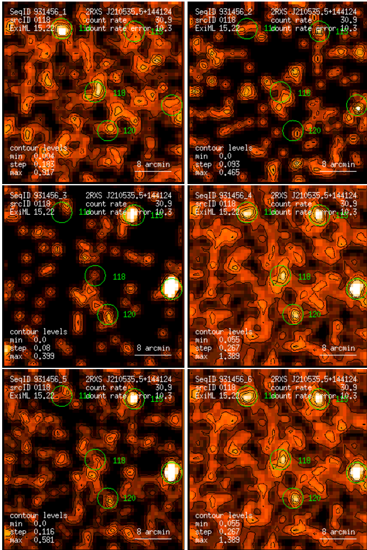
Figure 118: RASS 931456: detection 0118: band rate images, Gaussian filter: (1) PSPC channels 11 – 41, (2) 52 – 90, (3) 91 – 201, (4) 11 – 235, (5) 52 – 201, (6) 11 – 201. Broad band rates in counts/ks. Band rate contour levels in counts/ks/arcmin 2 .
