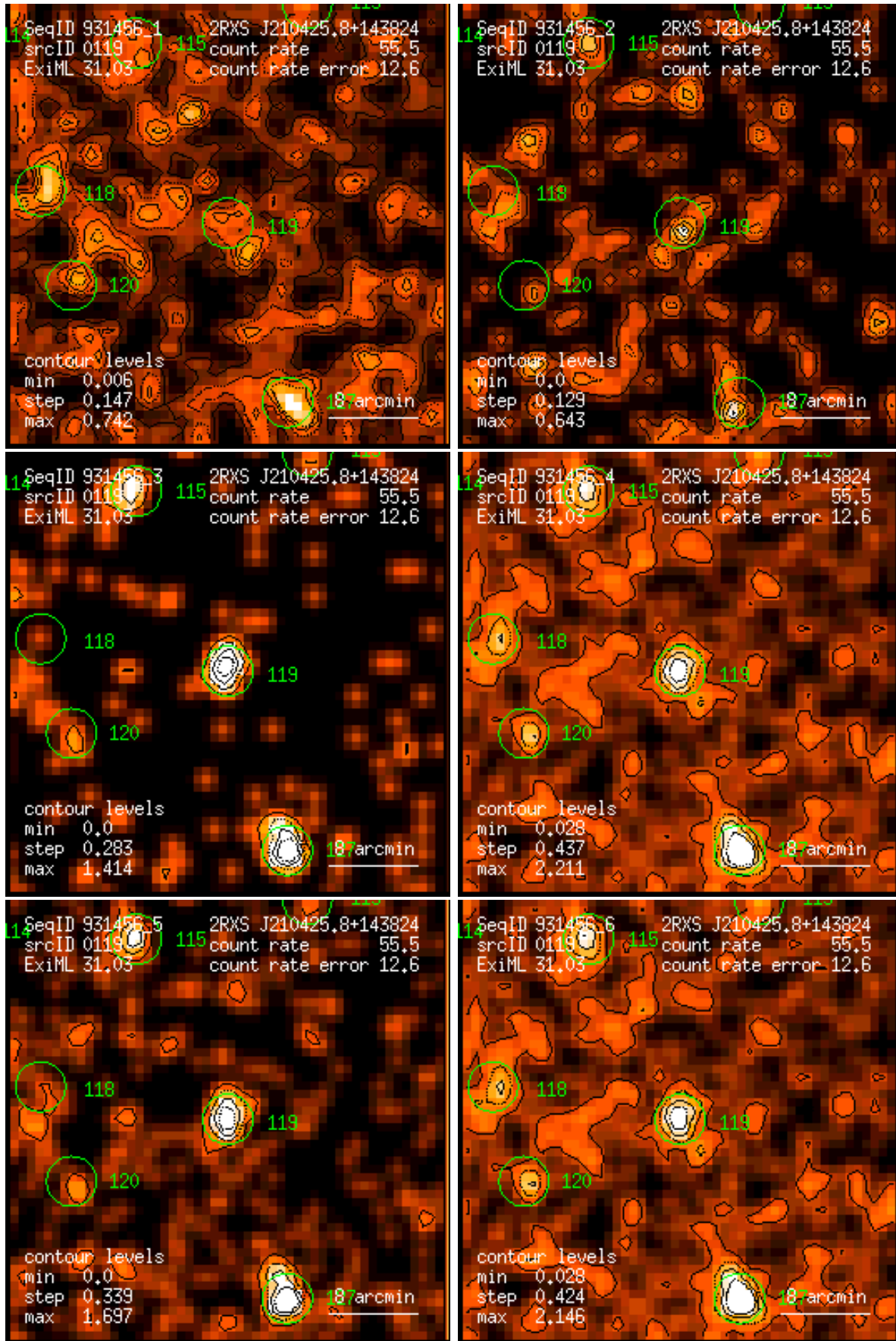
Figure 119: RASS 931456: detection 0119: band rate images, Gaussian filter: (1) PSPC channels 11 – 41, (2) 52 – 90, (3) 91 – 201, (4) 11 – 235, (5) 52 – 201, (6) 11 – 201. Broad band rates in counts/ks. Band rate contour levels in counts/ks/arcmin 2 .
