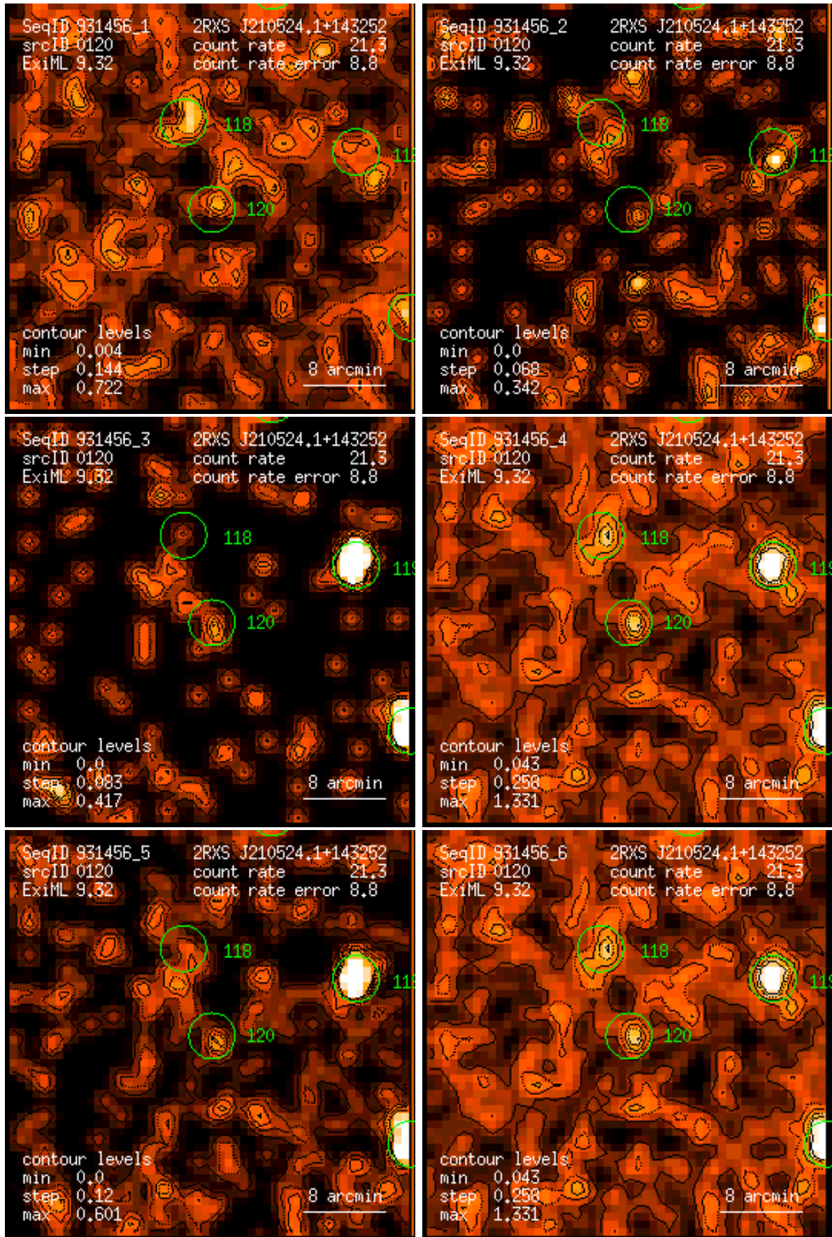
Figure 120: RASS 931456: detection 0120: band rate images, Gaussian filter: (1) PSPC channels 11 – 41, (2) 52 – 90, (3) 91 – 201, (4) 11 – 235, (5) 52 – 201, (6) 11 – 201. Broad band rates in counts/ks. Band rate contour levels in counts/ks/arcmin 2 .
