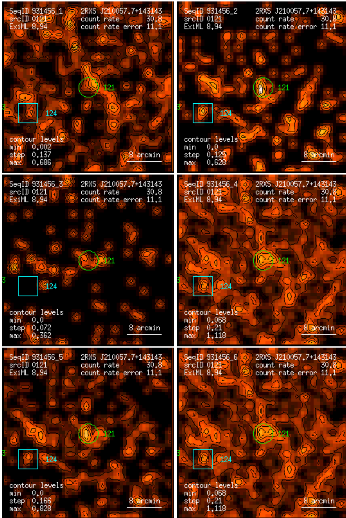
Figure 121: RASS 931456: detection 0121: band rate images, Gaussian filter: (1) PSPC channels 11 – 41, (2) 52 – 90, (3) 91 – 201, (4) 11 – 235, (5) 52 – 201, (6) 11 – 201. Broad band rates in counts/ks. Band rate contour levels in counts/ks/arcmin 2 .
