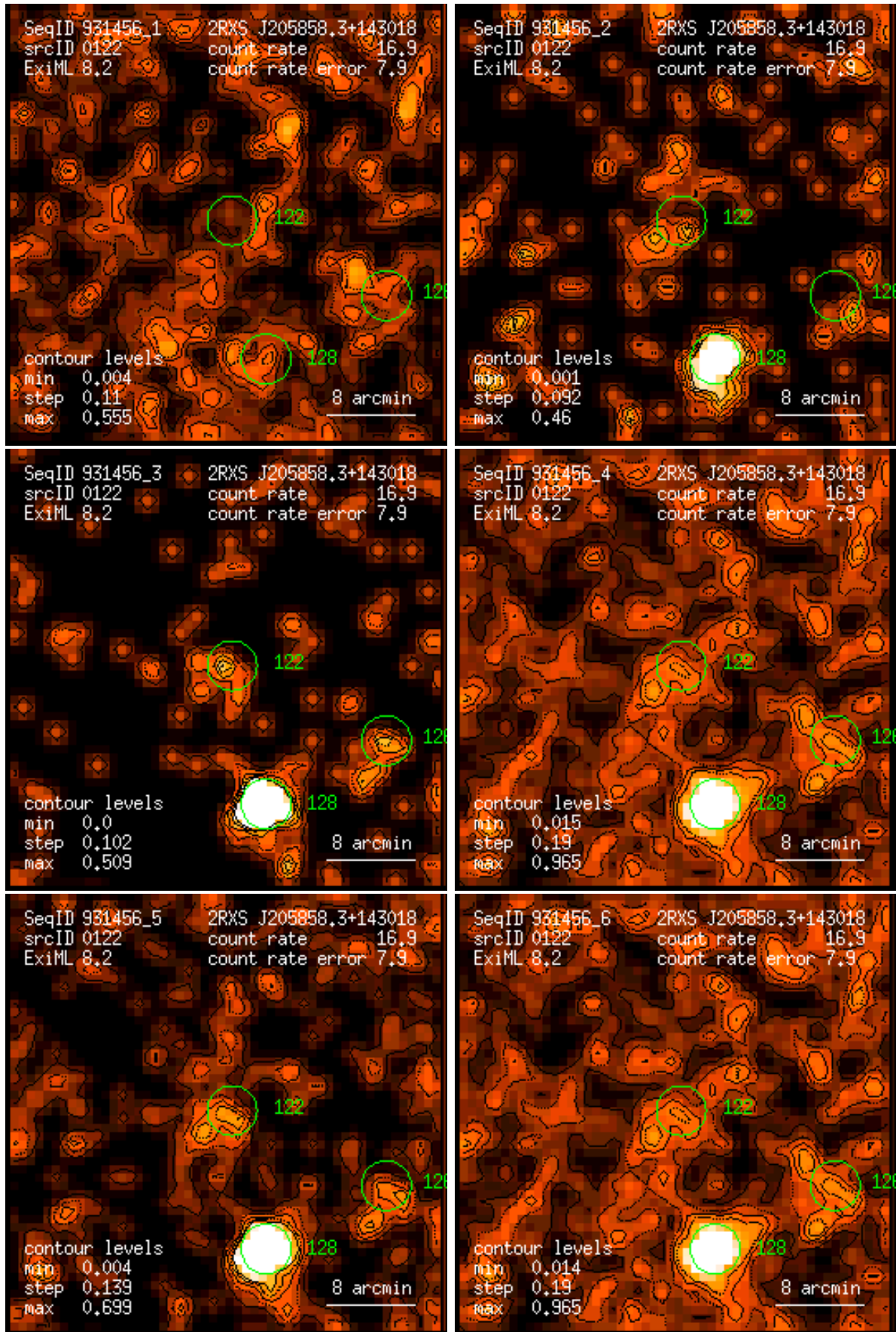
Figure 122: RASS 931456: detection 0122: band rate images, Gaussian filter: (1) PSPC channels 11 – 41, (2) 52 – 90, (3) 91 – 201, (4) 11 – 235, (5) 52 – 201, (6) 11 – 201. Broad band rates in counts/ks. Band rate contour levels in counts/ks/arcmin 2 .
