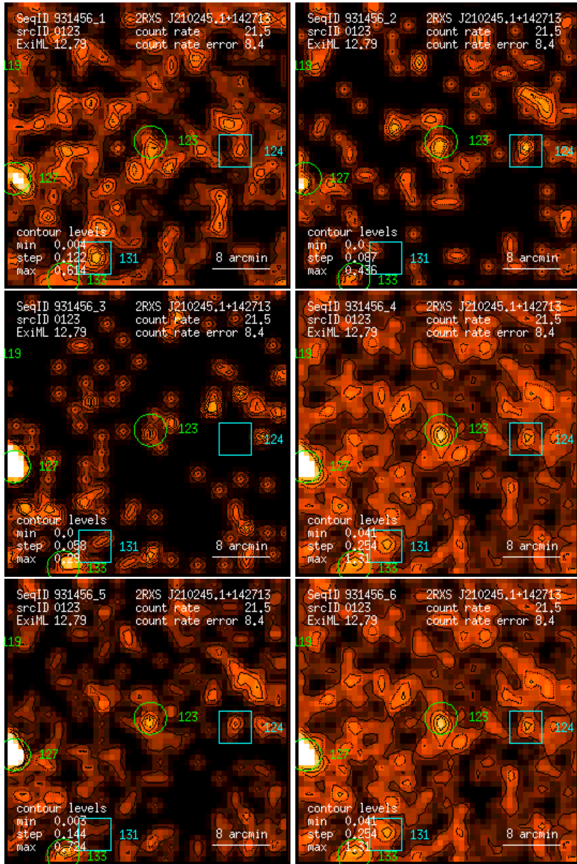
Figure 123: RASS 931456: detection 0123: band rate images, Gaussian filter: (1) PSPC channels 11 – 41, (2) 52 – 90, (3) 91 – 201, (4) 11 – 235, (5) 52 – 201, (6) 11 – 201. Broad band rates in counts/ks. Band rate contour levels in counts/ks/arcmin 2 .
