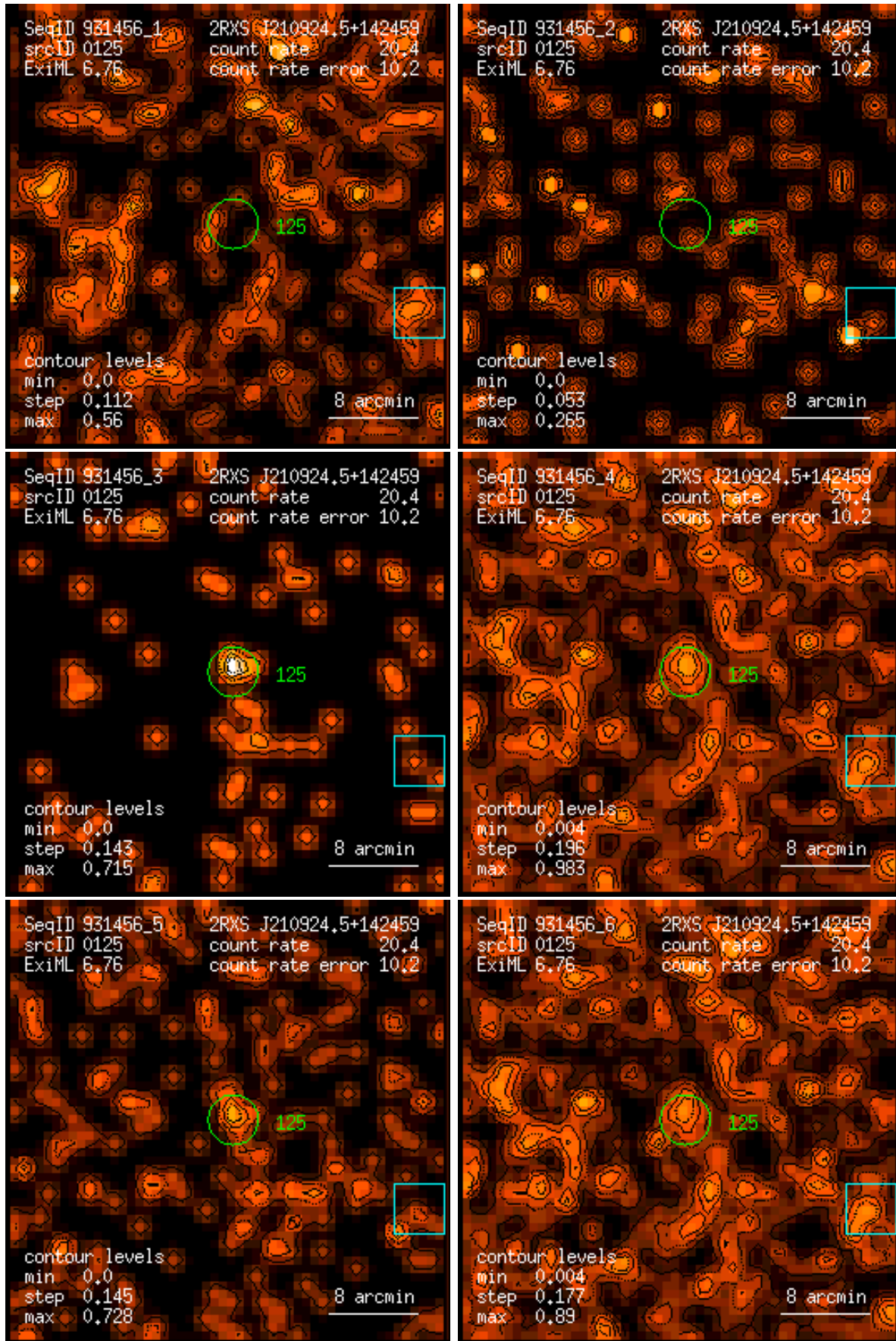
Figure 125: RASS 931456: detection 0125: band rate images, Gaussian filter: (1) PSPC channels 11 – 41, (2) 52 – 90, (3) 91 – 201, (4) 11 – 235, (5) 52 – 201, (6) 11 – 201. Broad band rates in counts/ks. Band rate contour levels in counts/ks/arcmin 2 .
