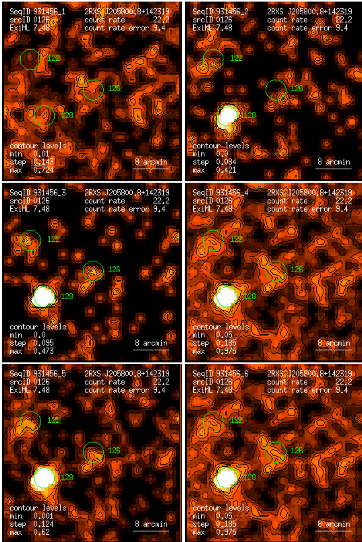
Figure 126: RASS 931456: detection 0126: band rate images, Gaussian filter: (1) PSPC channels 11 – 41, (2) 52 – 90, (3) 91 – 201, (4) 11 – 235, (5) 52 – 201, (6) 11 – 201. Broad band rates in counts/ks. Band rate contour levels in counts/ks/arcmin 2 .
