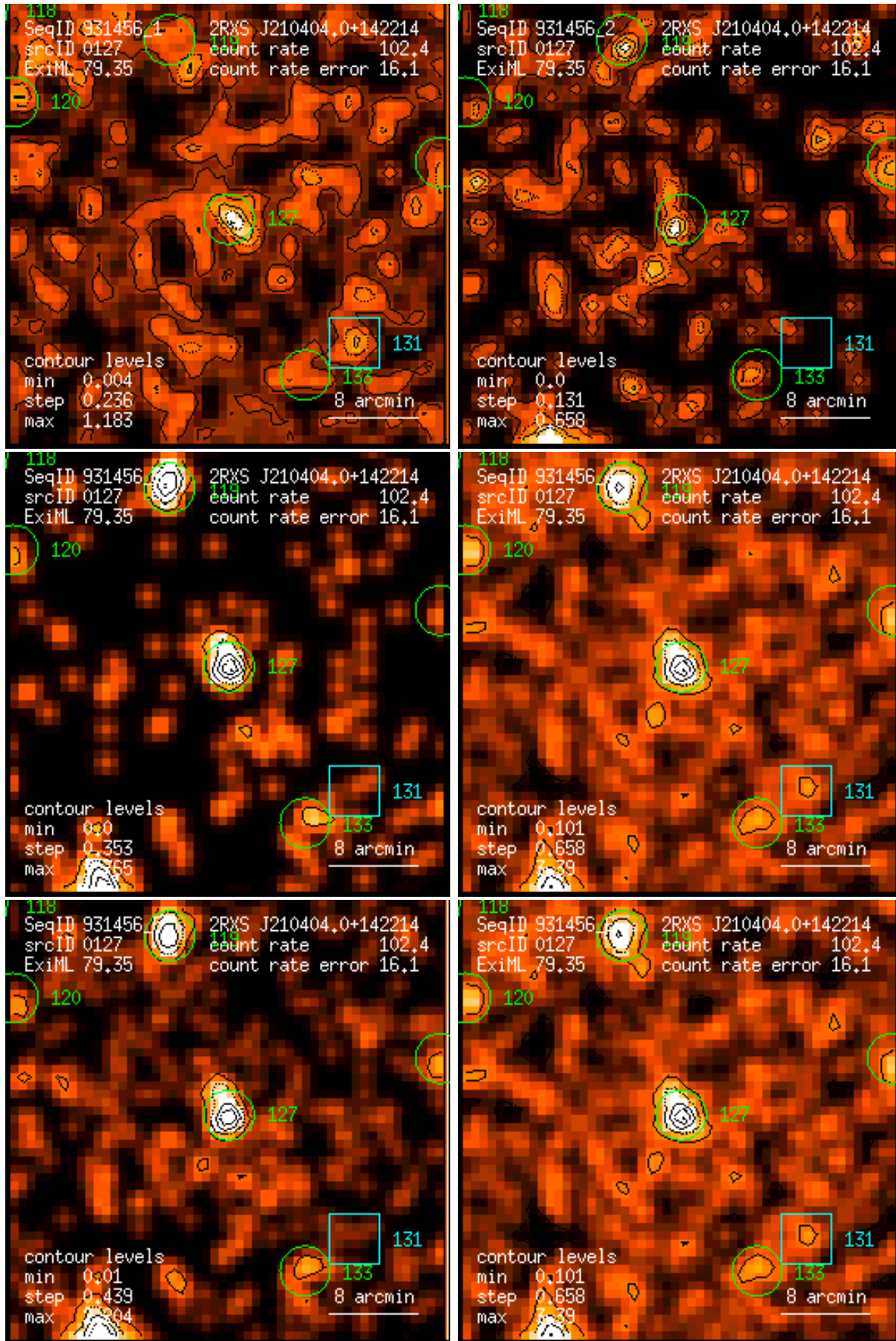
Figure 127: RASS 931456: detection 0127: band rate images, Gaussian filter: (1) PSPC channels 11 – 41, (2) 52 – 90, (3) 91 – 201, (4) 11 – 235, (5) 52 – 201, (6) 11 – 201. Broad band rates in counts/ks. Band rate contour levels in counts/ks/arcmin 2 .
