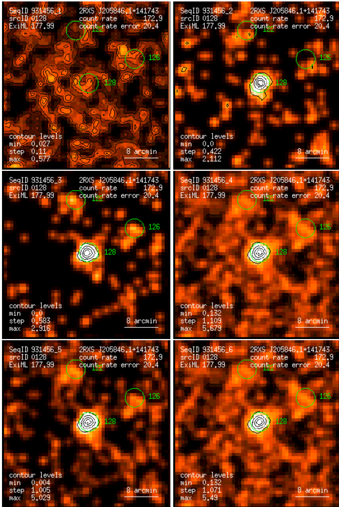
Figure 128: RASS 931456: detection 0128: band rate images, Gaussian filter: (1) PSPC channels 11 – 41, (2) 52 – 90, (3) 91 – 201, (4) 11 – 235, (5) 52 – 201, (6) 11 – 201. Broad band rates in counts/ks. Band rate contour levels in counts/ks/arcmin 2 .
