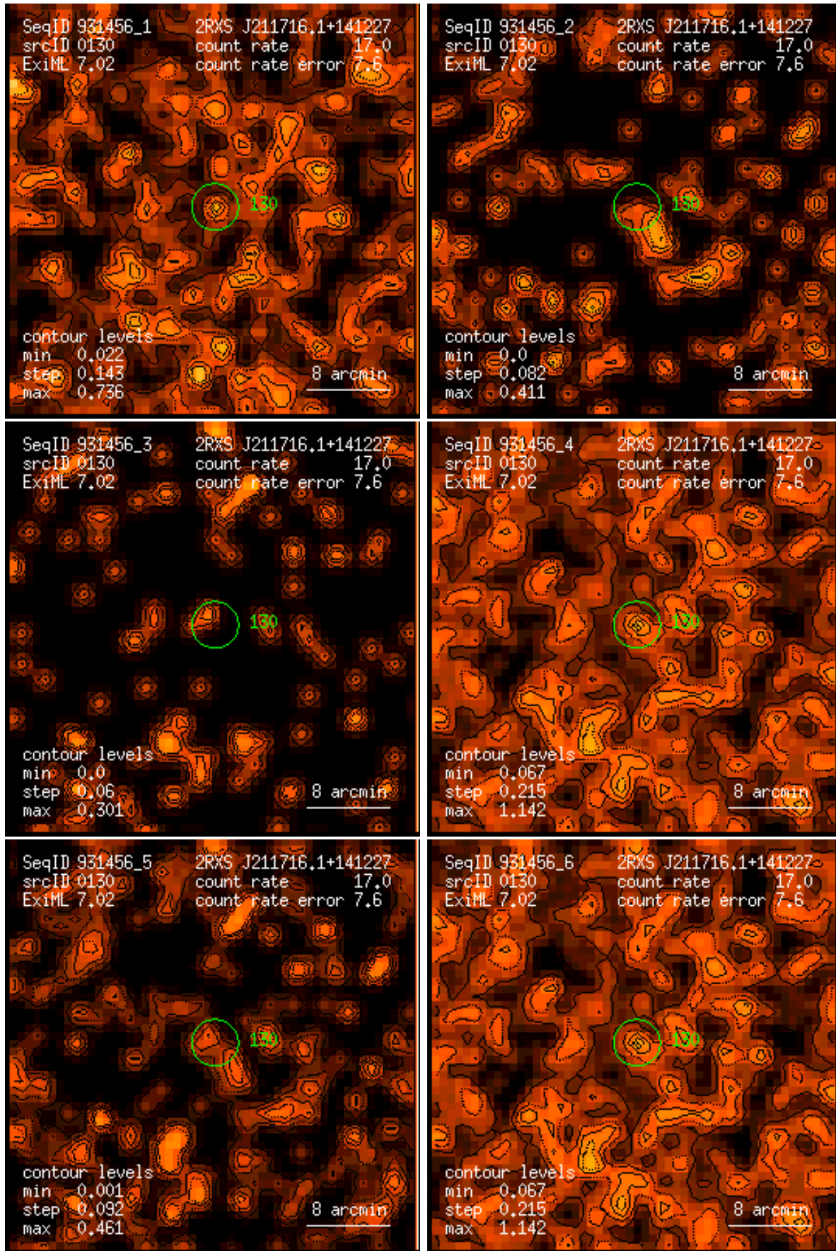
Figure 130: RASS 931456: detection 0130: band rate images, Gaussian filter: (1) PSPC channels 11 – 41, (2) 52 – 90, (3) 91 – 201, (4) 11 – 235, (5) 52 – 201, (6) 11 – 201. Broad band rates in counts/ks. Band rate contour levels in counts/ks/arcmin 2 .
