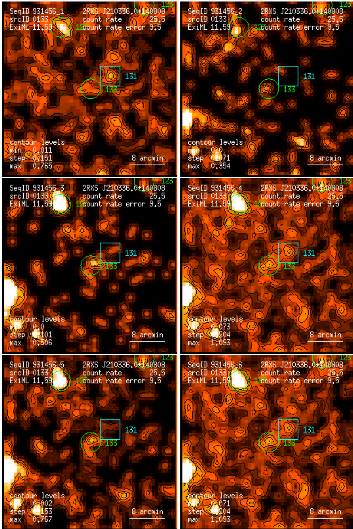
Figure 133: RASS 931456: detection 0133: band rate images, Gaussian filter: (1) PSPC channels 11 – 41, (2) 52 – 90, (3) 91 – 201, (4) 11 – 235, (5) 52 – 201, (6) 11 – 201. Broad band rates in counts/ks. Band rate contour levels in counts/ks/arcmin 2 .
