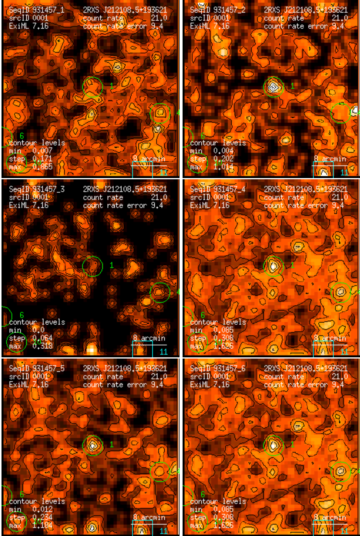
Figure 1: RASS 931457: detection 0001: band rate images, Gaussian filter: (1) PSPC channels 11 – 41, (2) 52 – 90, (3) 91 – 201, (4) 11 – 235, (5) 52 – 201, (6) 11 – 201. Broad band rates in counts/ks. Band rate contour levels in counts/ks/arcmin 2 .
