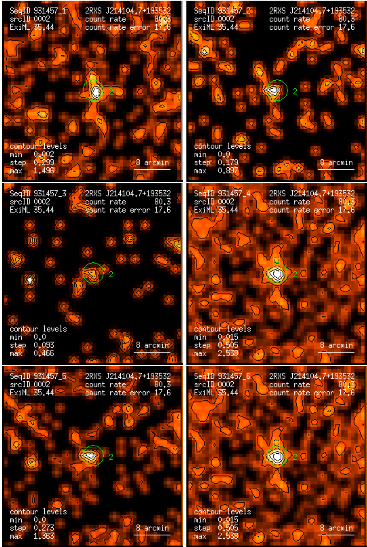
Figure 2: RASS 931457: detection 0002: band rate images, Gaussian filter: (1) PSPC channels 11 – 41, (2) 52 – 90, (3) 91 – 201, (4) 11 – 235, (5) 52 – 201, (6) 11 – 201. Broad band rates in counts/ks. Band rate contour levels in counts/ks/arcmin 2 .
