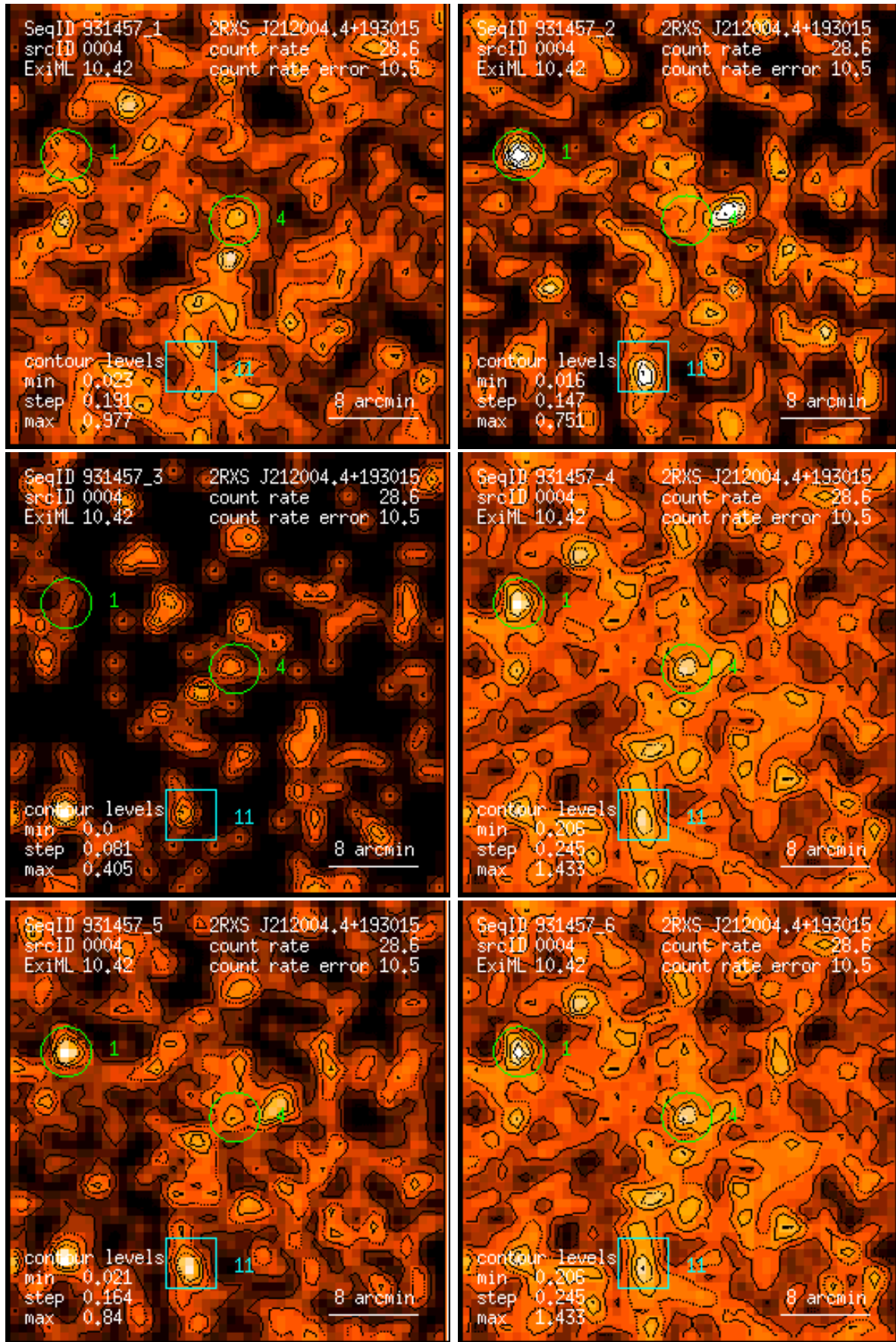
Figure 4: RASS 931457: detection 0004: band rate images, Gaussian filter: (1) PSPC channels 11 – 41, (2) 52 – 90, (3) 91 – 201, (4) 11 – 235, (5) 52 – 201, (6) 11 – 201. Broad band rates in counts/ks. Band rate contour levels in counts/ks/arcmin 2 .
