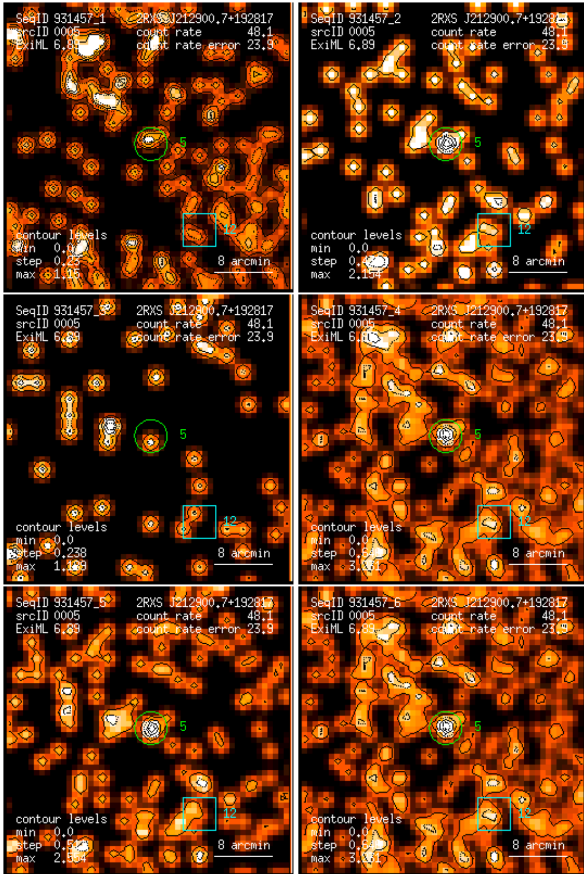
Figure 5: RASS 931457: detection 0005: band rate images, Gaussian filter: (1) PSPC channels 11 – 41, (2) 52 – 90, (3) 91 – 201, (4) 11 – 235, (5) 52 – 201, (6) 11 – 201. Broad band rates in counts/ks. Band rate contour levels in counts/ks/arcmin 2 .
