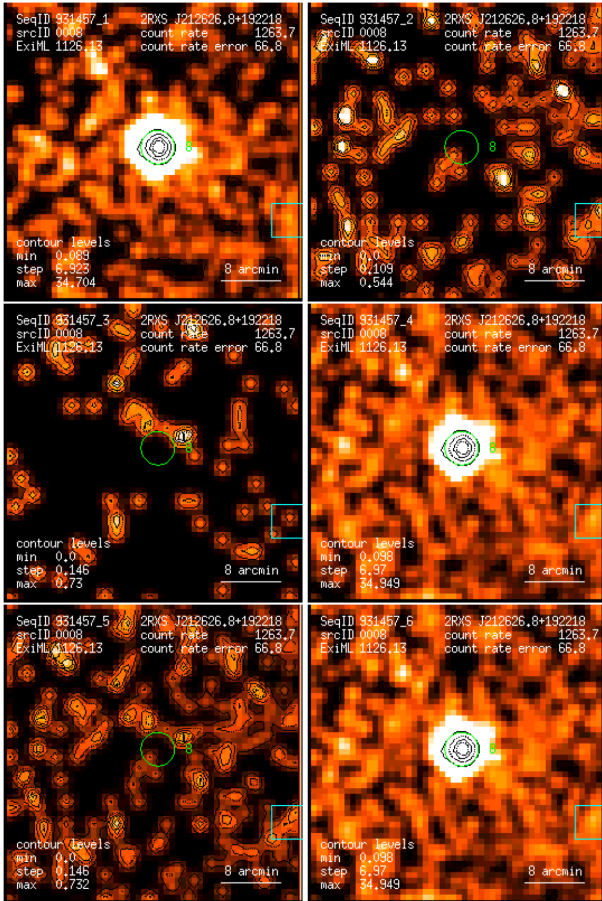
Figure 8: RASS 931457: detection 0008: band rate images, Gaussian filter: (1) PSPC channels 11 – 41, (2) 52 – 90, (3) 91 – 201, (4) 11 – 235, (5) 52 – 201, (6) 11 – 201. Broad band rates in counts/ks. Band rate contour levels in counts/ks/arcmin 2 .
