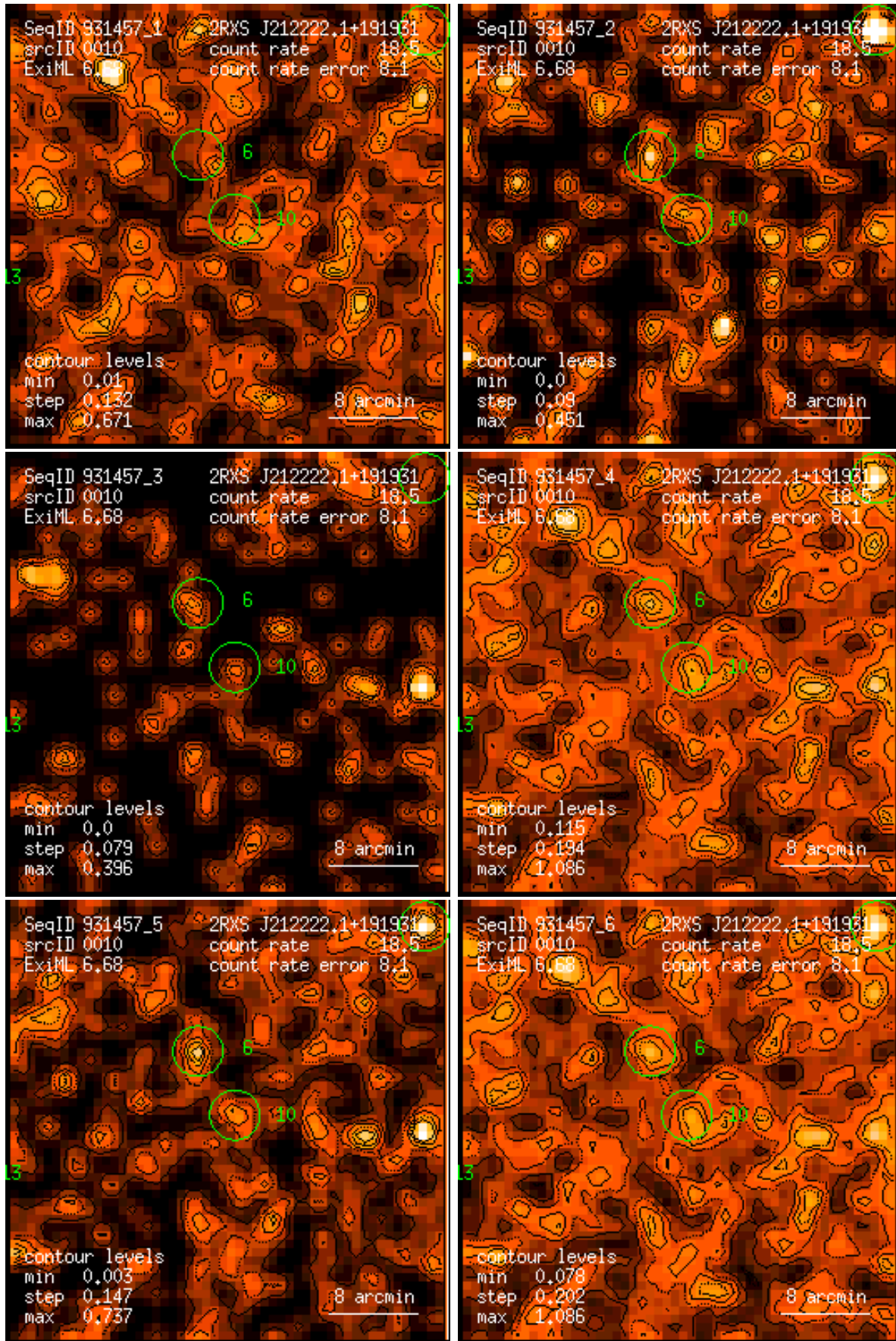
Figure 10: RASS 931457: detection 0010: band rate images, Gaussian filter: (1) PSPC channels 11 – 41, (2) 52 – 90, (3) 91 – 201, (4) 11 – 235, (5) 52 – 201, (6) 11 – 201. Broad band rates in counts/ks. Band rate contour levels in counts/ks/arcmin 2 .
