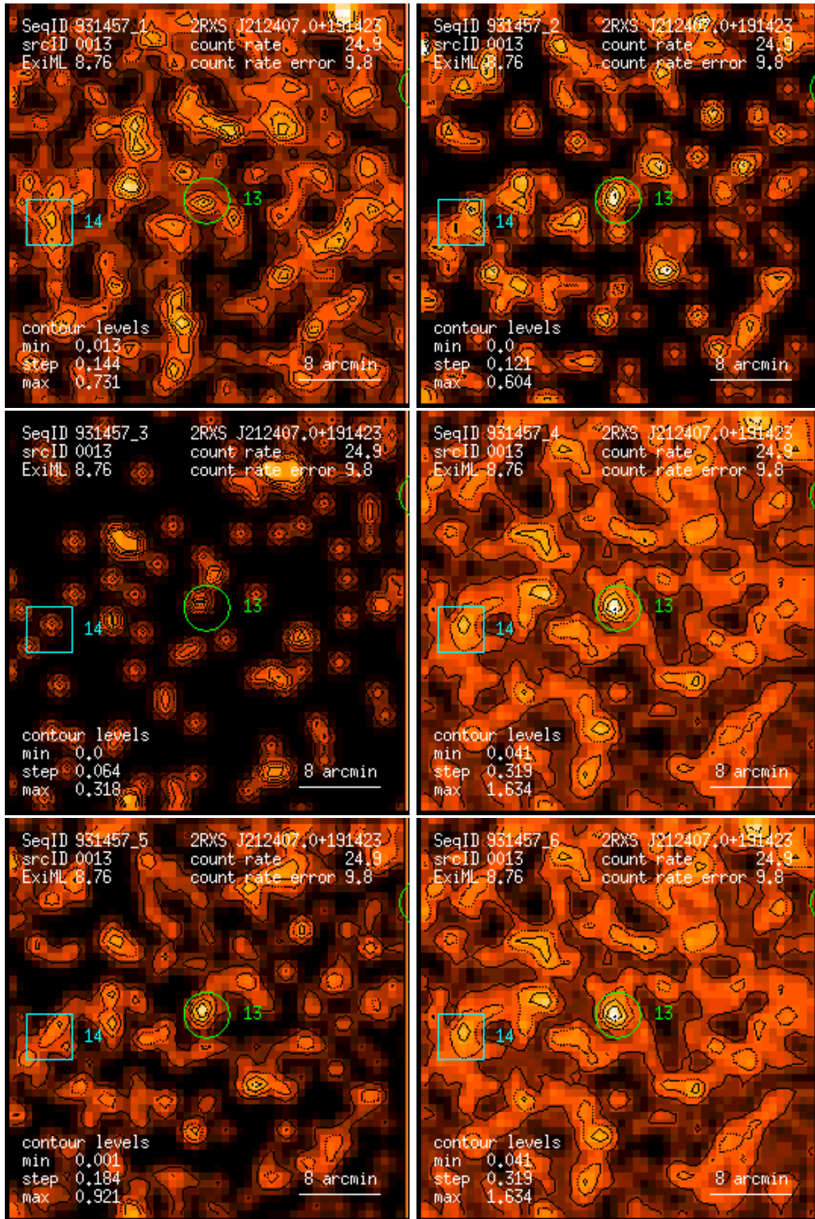
Figure 13: RASS 931457: detection 0013: band rate images, Gaussian filter: (1) PSPC channels 11 – 41, (2) 52 – 90, (3) 91 – 201, (4) 11 – 235, (5) 52 – 201, (6) 11 – 201. Broad band rates in counts/ks. Band rate contour levels in counts/ks/arcmin 2 .
