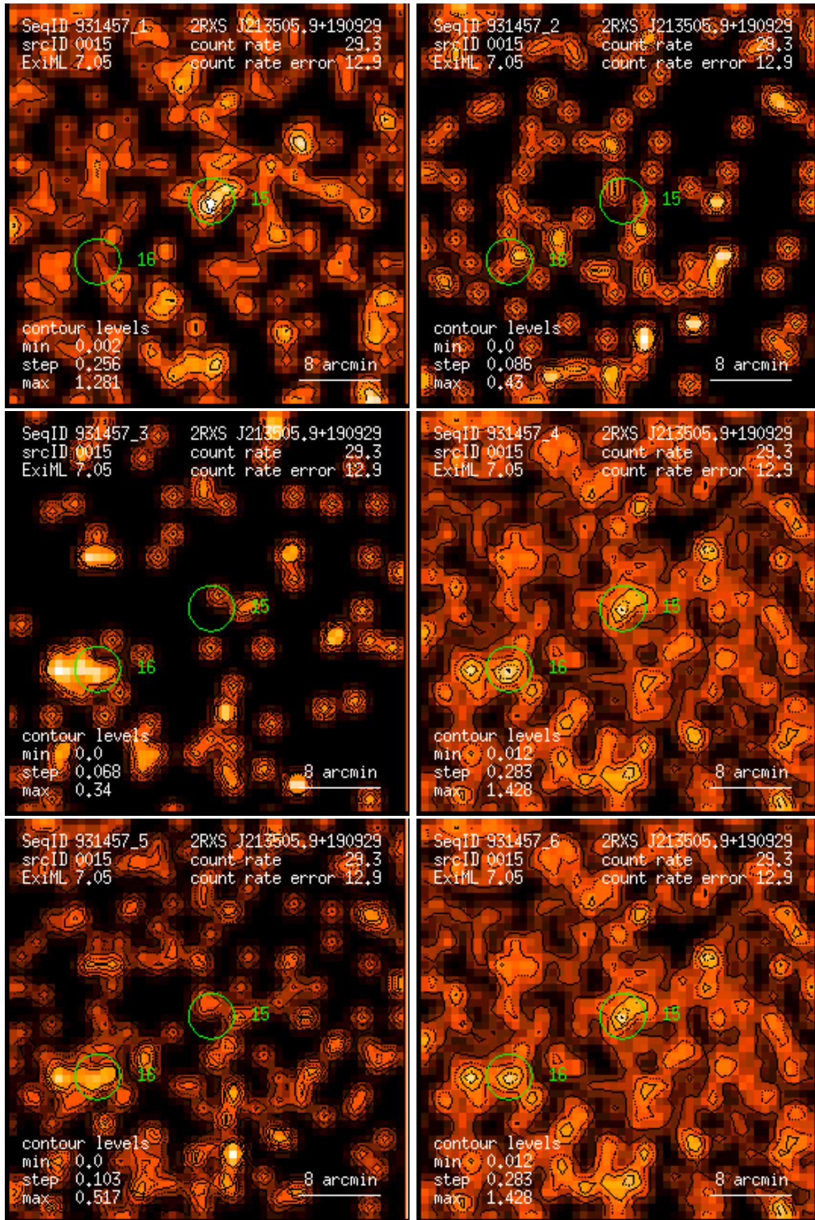
Figure 15: RASS 931457: detection 0015: band rate images, Gaussian filter: (1) PSPC channels 11 – 41, (2) 52 – 90, (3) 91 – 201, (4) 11 – 235, (5) 52 – 201, (6) 11 – 201. Broad band rates in counts/ks. Band rate contour levels in counts/ks/arcmin 2 .
