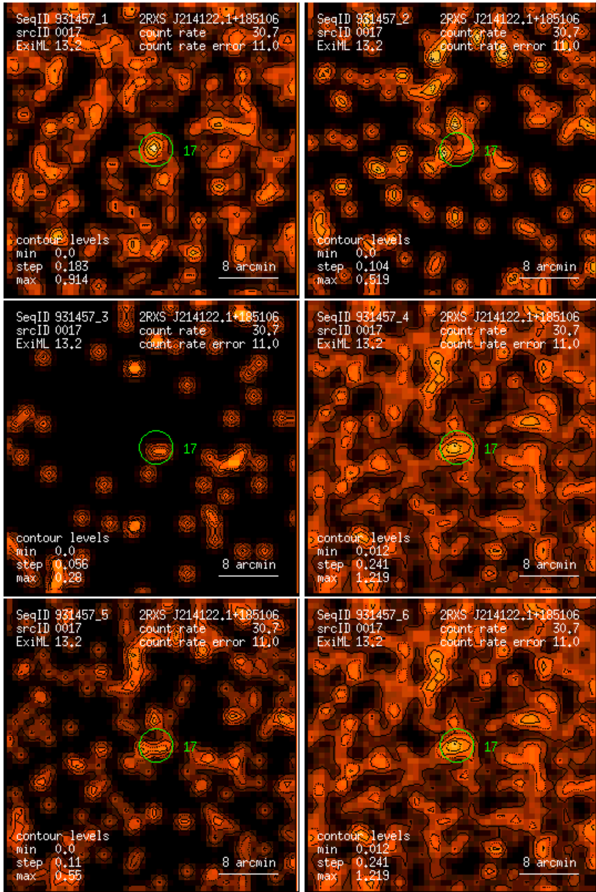
Figure 17: RASS 931457: detection 0017: band rate images, Gaussian filter: (1) PSPC channels 11 – 41, (2) 52 – 90, (3) 91 – 201, (4) 11 – 235, (5) 52 – 201, (6) 11 – 201. Broad band rates in counts/ks. Band rate contour levels in counts/ks/arcmin 2 .
