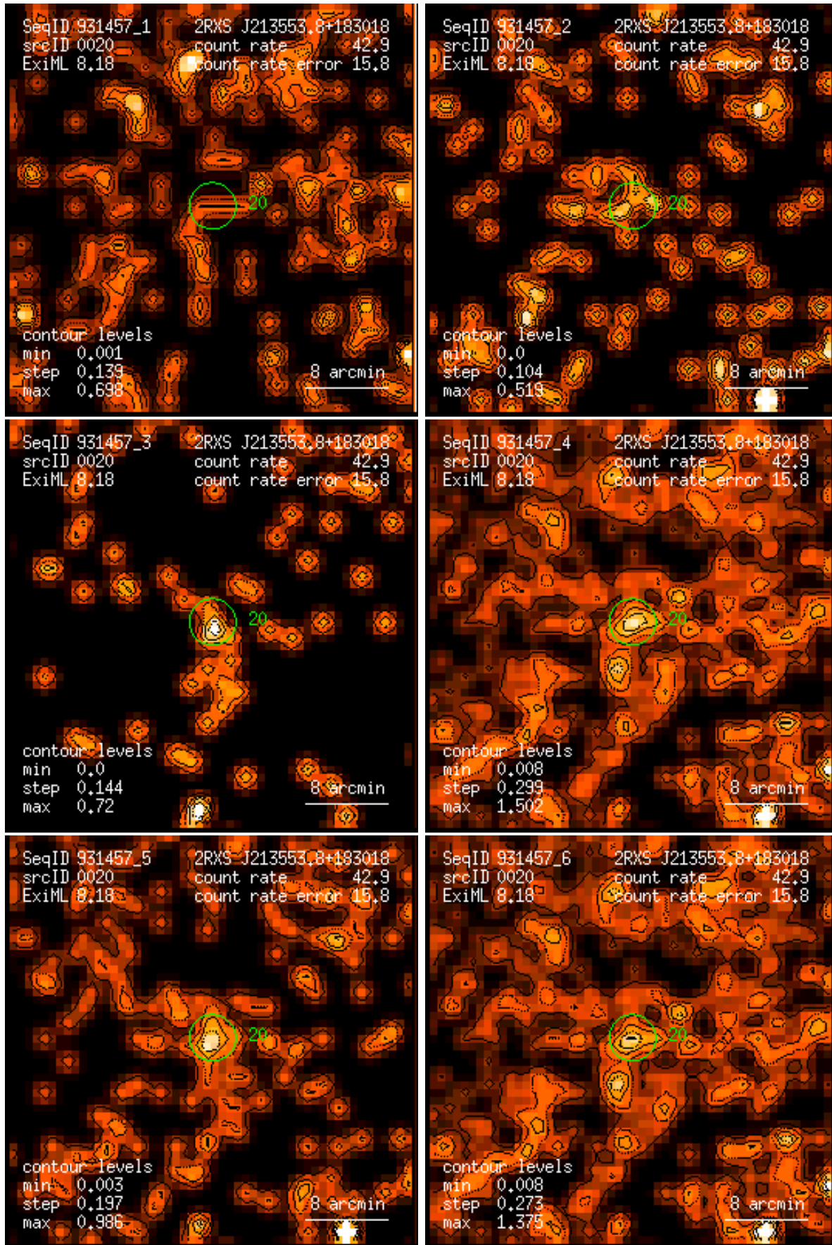
Figure 20: RASS 931457: detection 0020: band rate images, Gaussian filter: (1) PSPC channels 11 – 41, (2) 52 – 90, (3) 91 – 201, (4) 11 – 235, (5) 52 – 201, (6) 11 – 201. Broad band rates in counts/ks. Band rate contour levels in counts/ks/arcmin 2 .
