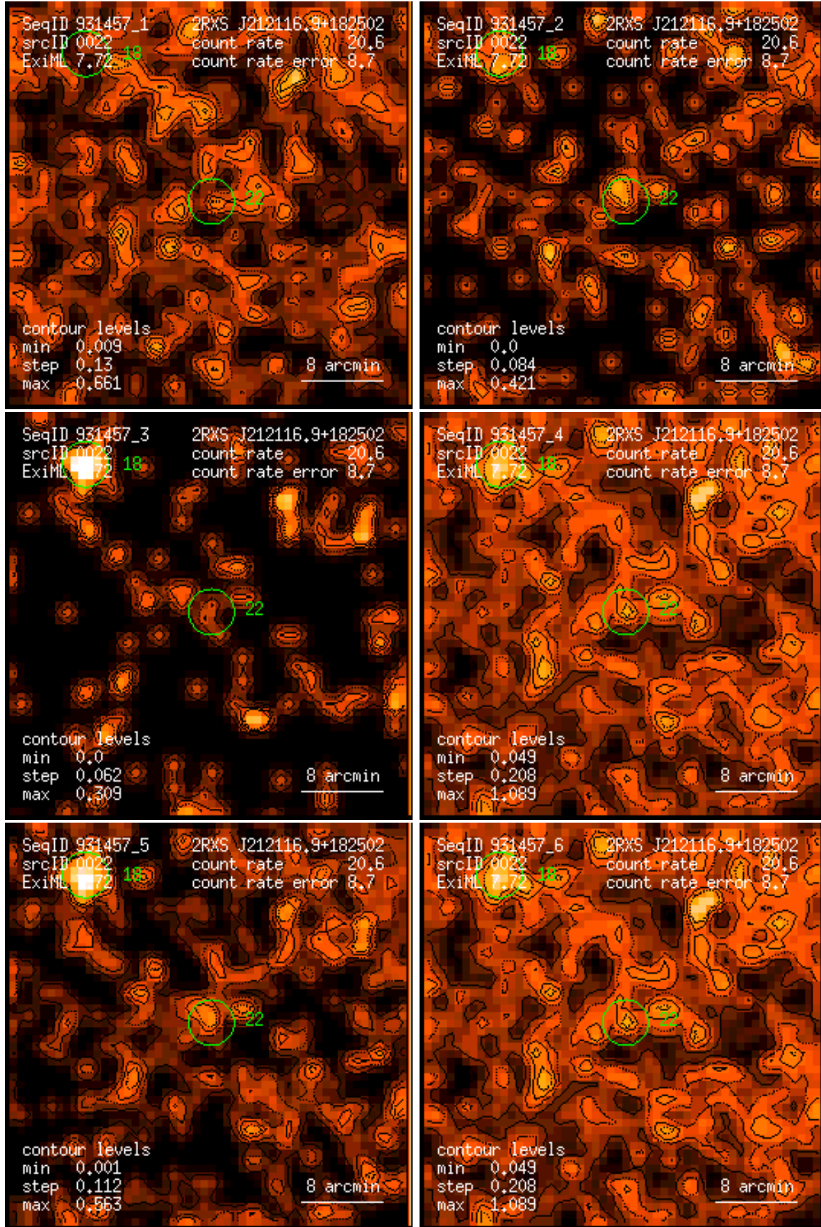
Figure 22: RASS 931457: detection 0022: band rate images, Gaussian filter: (1) PSPC channels 11 – 41, (2) 52 – 90, (3) 91 – 201, (4) 11 – 235, (5) 52 – 201, (6) 11 – 201. Broad band rates in counts/ks. Band rate contour levels in counts/ks/arcmin 2 .
