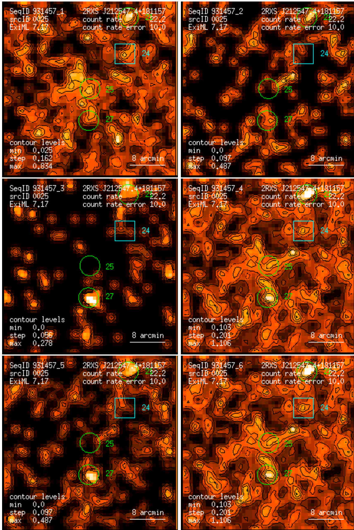
Figure 25: RASS 931457: detection 0025: band rate images, Gaussian filter: (1) PSPC channels 11 – 41, (2) 52 – 90, (3) 91 – 201, (4) 11 – 235, (5) 52 – 201, (6) 11 – 201. Broad band rates in counts/ks. Band rate contour levels in counts/ks/arcmin 2 .
