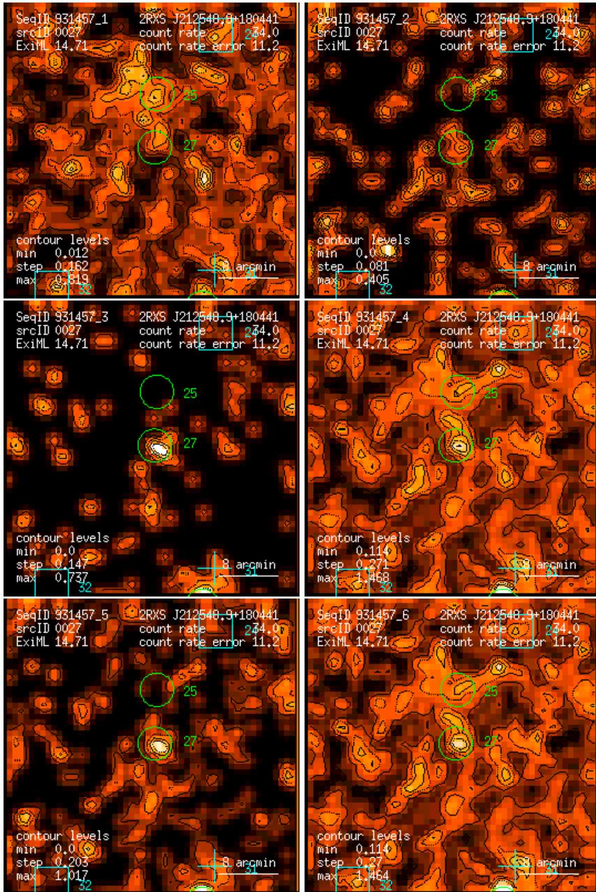
Figure 27: RASS 931457: detection 0027: band rate images, Gaussian filter: (1) PSPC channels 11 – 41, (2) 52 – 90, (3) 91 – 201, (4) 11 – 235, (5) 52 – 201, (6) 11 – 201. Broad band rates in counts/ks. Band rate contour levels in counts/ks/arcmin 2 .
