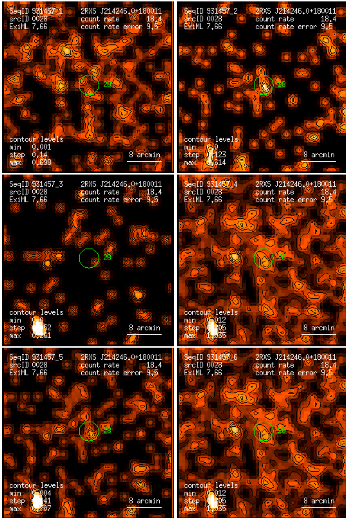
Figure 28: RASS 931457: detection 0028: band rate images, Gaussian filter: (1) PSPC channels 11 – 41, (2) 52 – 90, (3) 91 – 201, (4) 11 – 235, (5) 52 – 201, (6) 11 – 201. Broad band rates in counts/ks. Band rate contour levels in counts/ks/arcmin 2 .
