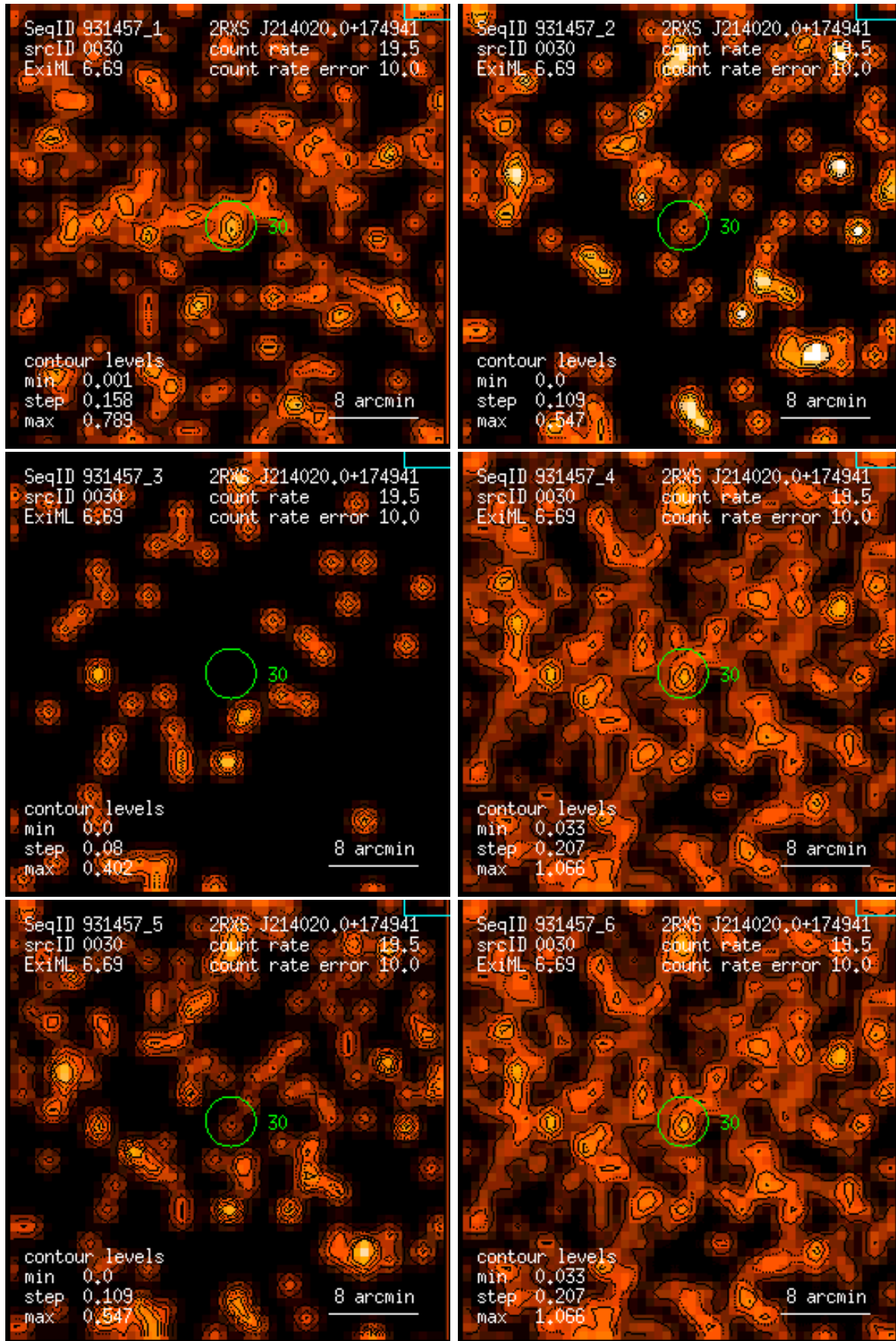
Figure 30: RASS 931457: detection 0030: band rate images, Gaussian filter: (1) PSPC channels 11 – 41, (2) 52 – 90, (3) 91 – 201, (4) 11 – 235, (5) 52 – 201, (6) 11 – 201. Broad band rates in counts/ks. Band rate contour levels in counts/ks/arcmin 2 .
