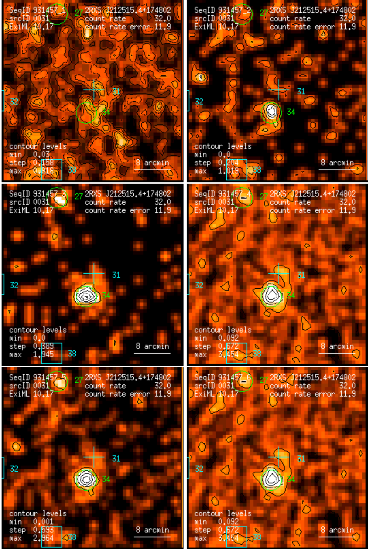
Figure 31: RASS 931457: detection 0031: band rate images, Gaussian filter: (1) PSPC channels 11 – 41, (2) 52 – 90, (3) 91 – 201, (4) 11 – 235, (5) 52 – 201, (6) 11 – 201. Broad band rates in counts/ks. Band rate contour levels in counts/ks/arcmin 2 .
