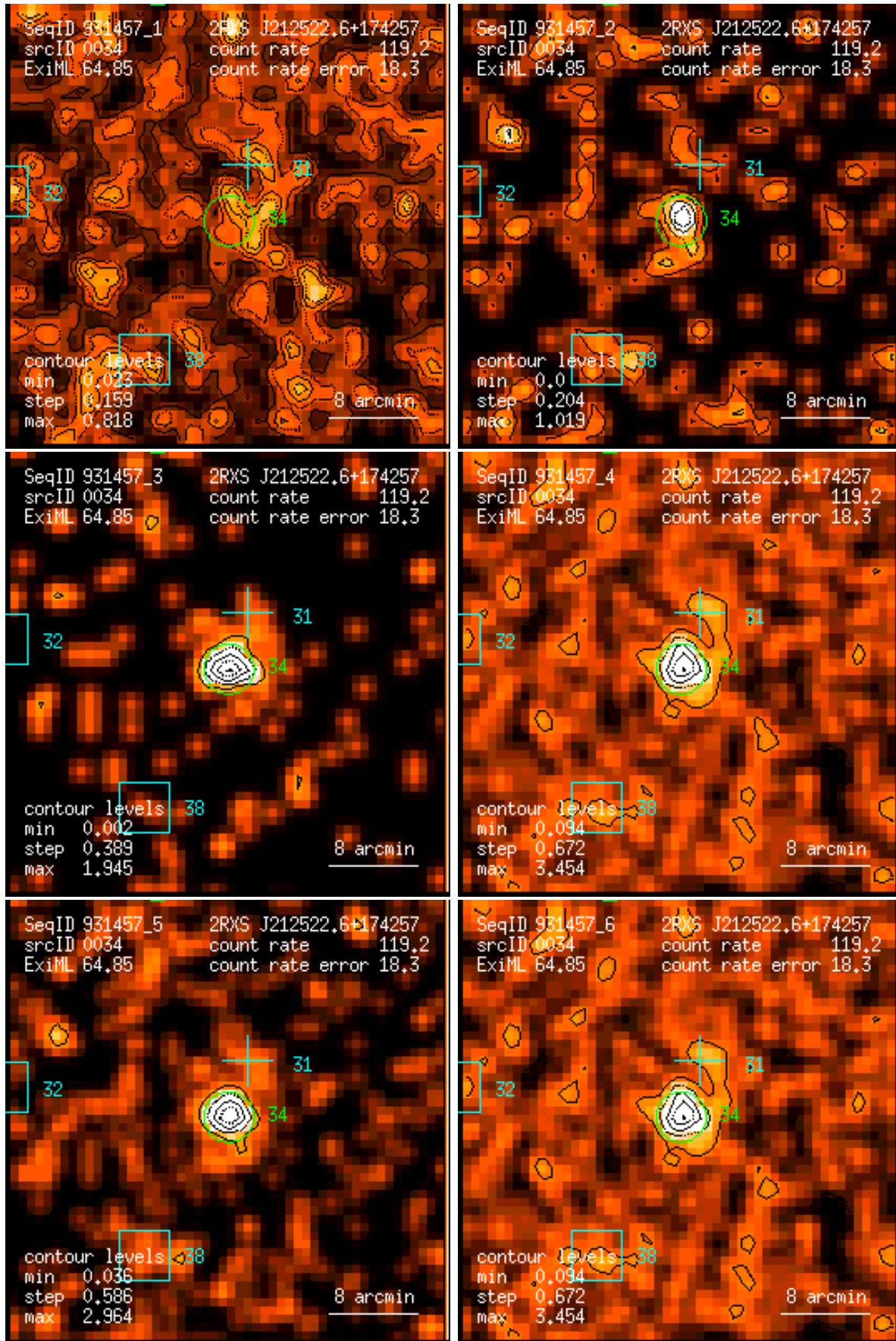
Figure 34: RASS 931457: detection 0034: band rate images, Gaussian filter: (1) PSPC channels 11 – 41, (2) 52 – 90, (3) 91 – 201, (4) 11 – 235, (5) 52 – 201, (6) 11 – 201. Broad band rates in counts/ks. Band rate contour levels in counts/ks/arcmin 2 .
