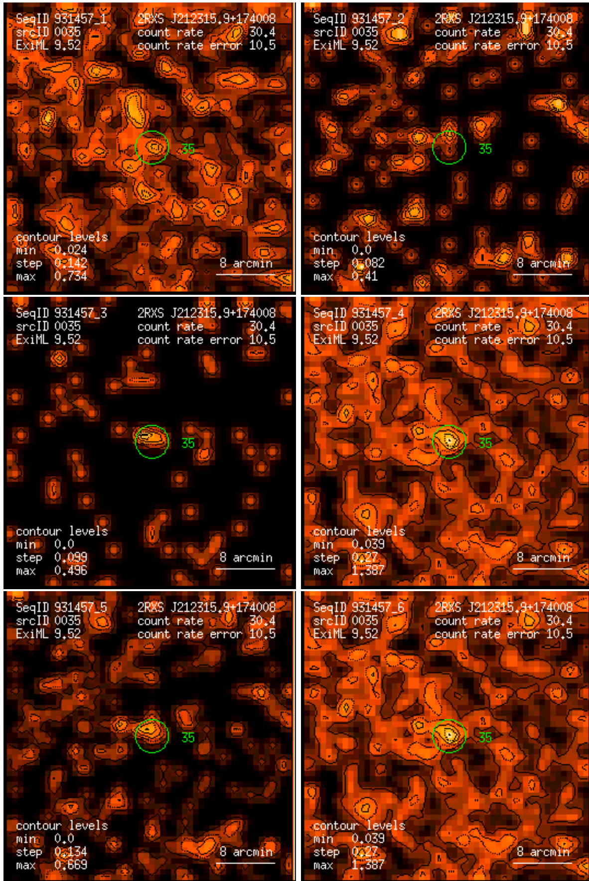
Figure 35: RASS 931457: detection 0035: band rate images, Gaussian filter: (1) PSPC channels 11 – 41, (2) 52 – 90, (3) 91 – 201, (4) 11 – 235, (5) 52 – 201, (6) 11 – 201. Broad band rates in counts/ks. Band rate contour levels in counts/ks/arcmin 2 .
