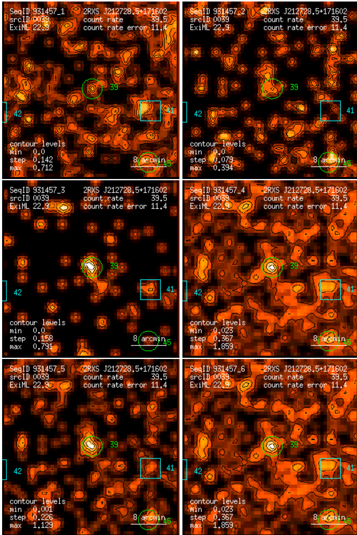
Figure 39: RASS 931457: detection 0039: band rate images, Gaussian filter: (1) PSPC channels 11 – 41, (2) 52 – 90, (3) 91 – 201, (4) 11 – 235, (5) 52 – 201, (6) 11 – 201. Broad band rates in counts/ks. Band rate contour levels in counts/ks/arcmin 2 .
