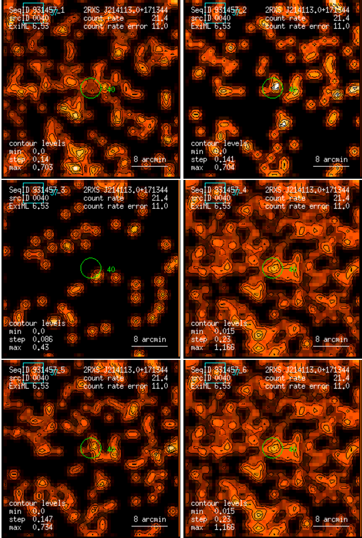
Figure 40: RASS 931457: detection 0040: band rate images, Gaussian filter: (1) PSPC channels 11 – 41, (2) 52 – 90, (3) 91 – 201, (4) 11 – 235, (5) 52 – 201, (6) 11 – 201. Broad band rates in counts/ks. Band rate contour levels in counts/ks/arcmin 2 .
