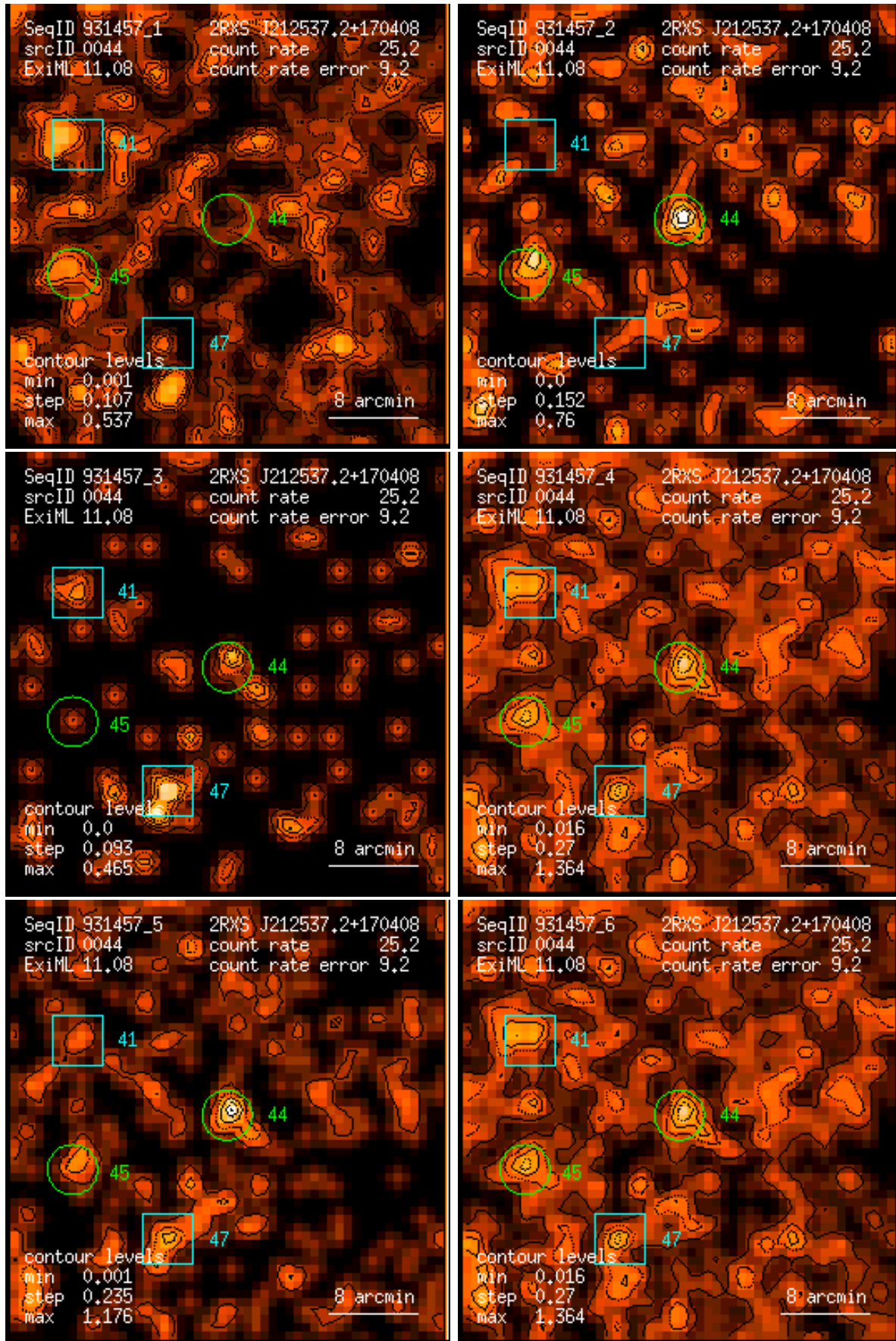
Figure 44: RASS 931457: detection 0044: band rate images, Gaussian filter: (1) PSPC channels 11 – 41, (2) 52 – 90, (3) 91 – 201, (4) 11 – 235, (5) 52 – 201, (6) 11 – 201. Broad band rates in counts/ks. Band rate contour levels in counts/ks/arcmin 2 .
