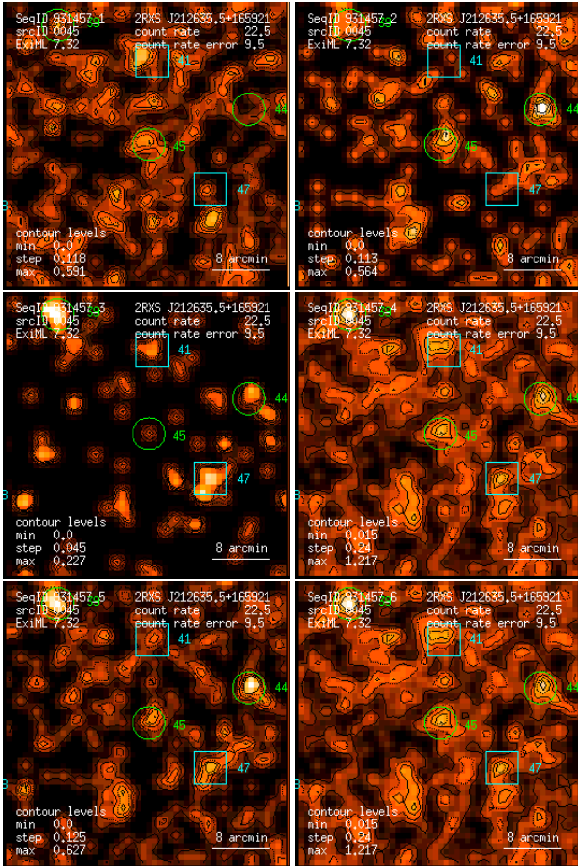
Figure 45: RASS 931457: detection 0045: band rate images, Gaussian filter: (1) PSPC channels 11 – 41, (2) 52 – 90, (3) 91 – 201, (4) 11 – 235, (5) 52 – 201, (6) 11 – 201. Broad band rates in counts/ks. Band rate contour levels in counts/ks/arcmin 2 .
