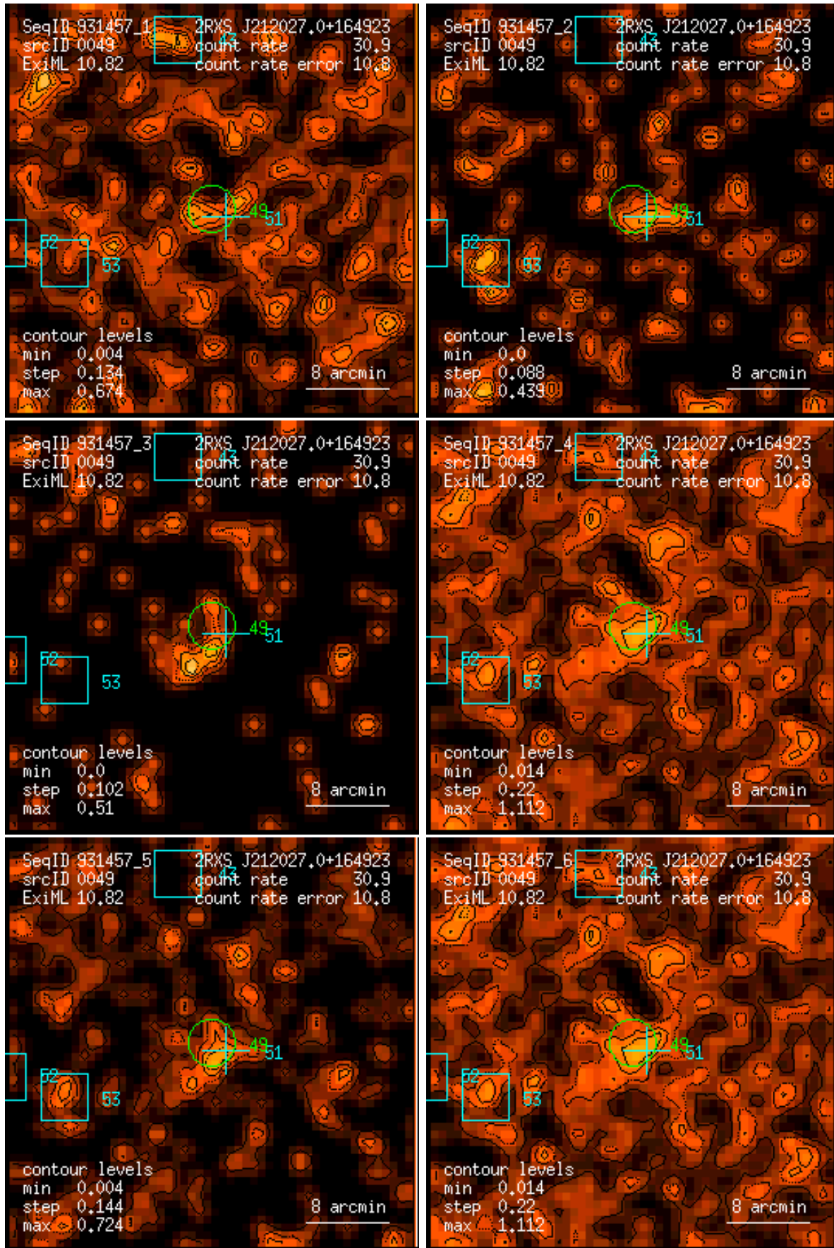
Figure 49: RASS 931457: detection 0049: band rate images, Gaussian filter: (1) PSPC channels 11 – 41, (2) 52 – 90, (3) 91 – 201, (4) 11 – 235, (5) 52 – 201, (6) 11 – 201. Broad band rates in counts/ks. Band rate contour levels in counts/ks/arcmin 2 .
