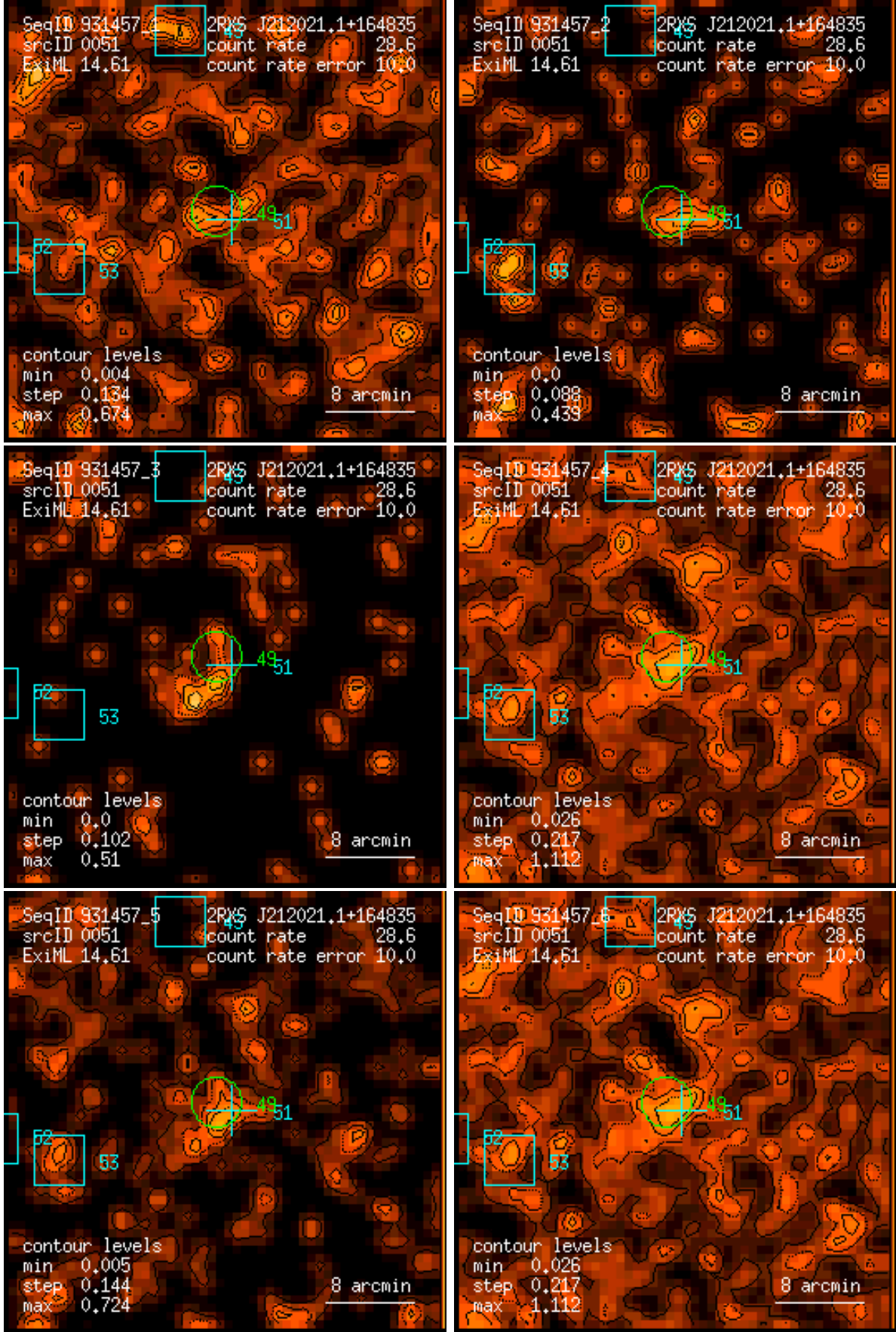
Figure 51: RASS 931457: detection 0051: band rate images, Gaussian filter: (1) PSPC channels 11 – 41, (2) 52 – 90, (3) 91 – 201, (4) 11 – 235, (5) 52 – 201, (6) 11 – 201. Broad band rates in counts/ks. Band rate contour levels in counts/ks/arcmin 2 .
