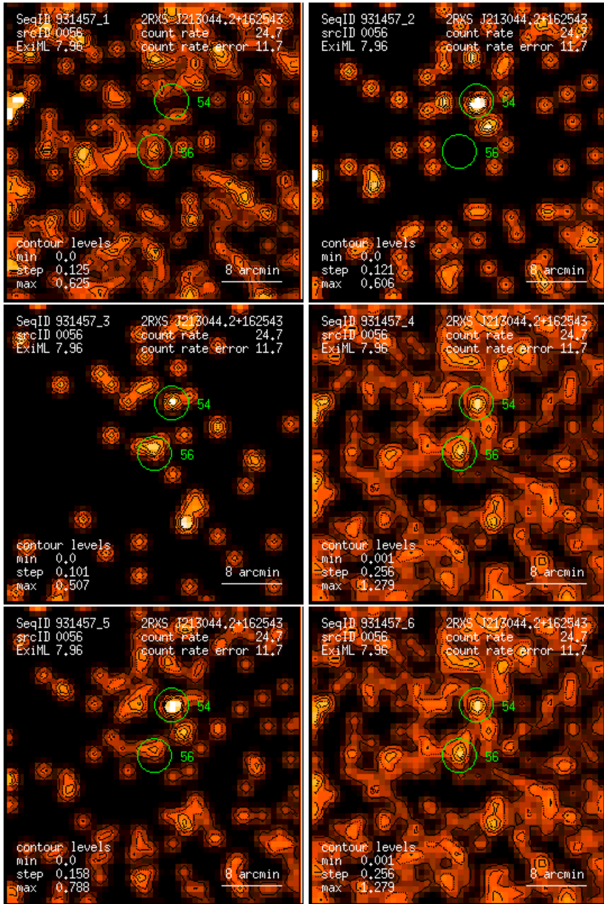
Figure 56: RASS 931457: detection 0056: band rate images, Gaussian filter: (1) PSPC channels 11 – 41, (2) 52 – 90, (3) 91 – 201, (4) 11 – 235, (5) 52 – 201, (6) 11 – 201. Broad band rates in counts/ks. Band rate contour levels in counts/ks/arcmin 2 .
