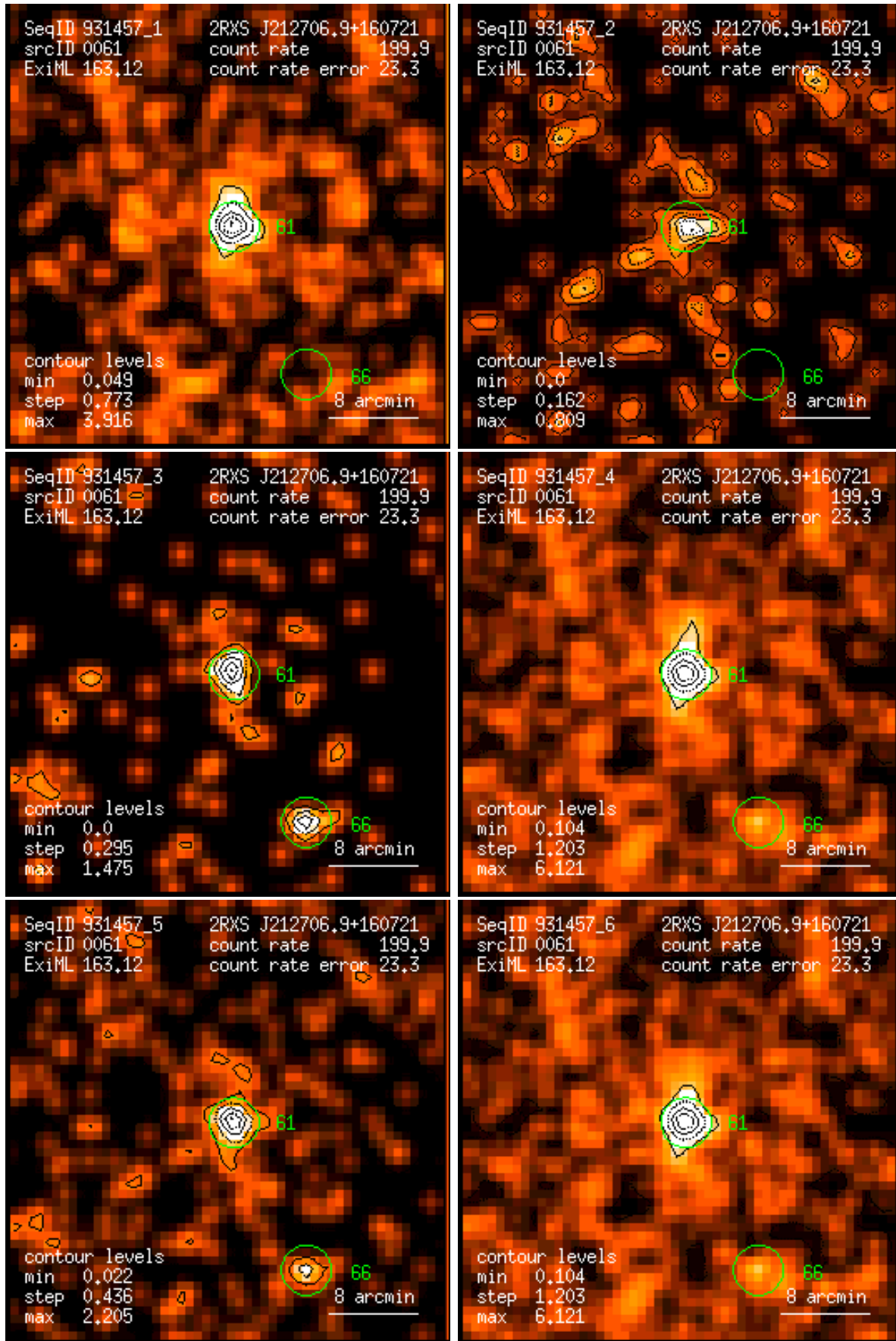
Figure 61: RASS 931457: detection 0061: band rate images, Gaussian filter: (1) PSPC channels 11 – 41, (2) 52 – 90, (3) 91 – 201, (4) 11 – 235, (5) 52 – 201, (6) 11 – 201. Broad band rates in counts/ks. Band rate contour levels in counts/ks/arcmin 2 .
