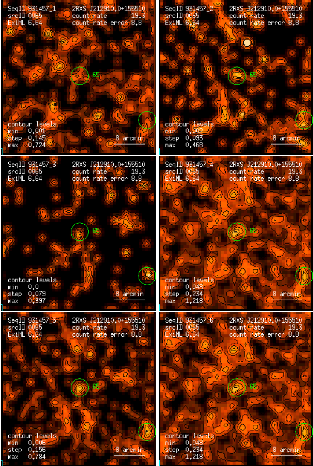
Figure 65: RASS 931457: detection 0065: band rate images, Gaussian filter: (1) PSPC channels 11 – 41, (2) 52 – 90, (3) 91 – 201, (4) 11 – 235, (5) 52 – 201, (6) 11 – 201. Broad band rates in counts/ks. Band rate contour levels in counts/ks/arcmin 2 .
