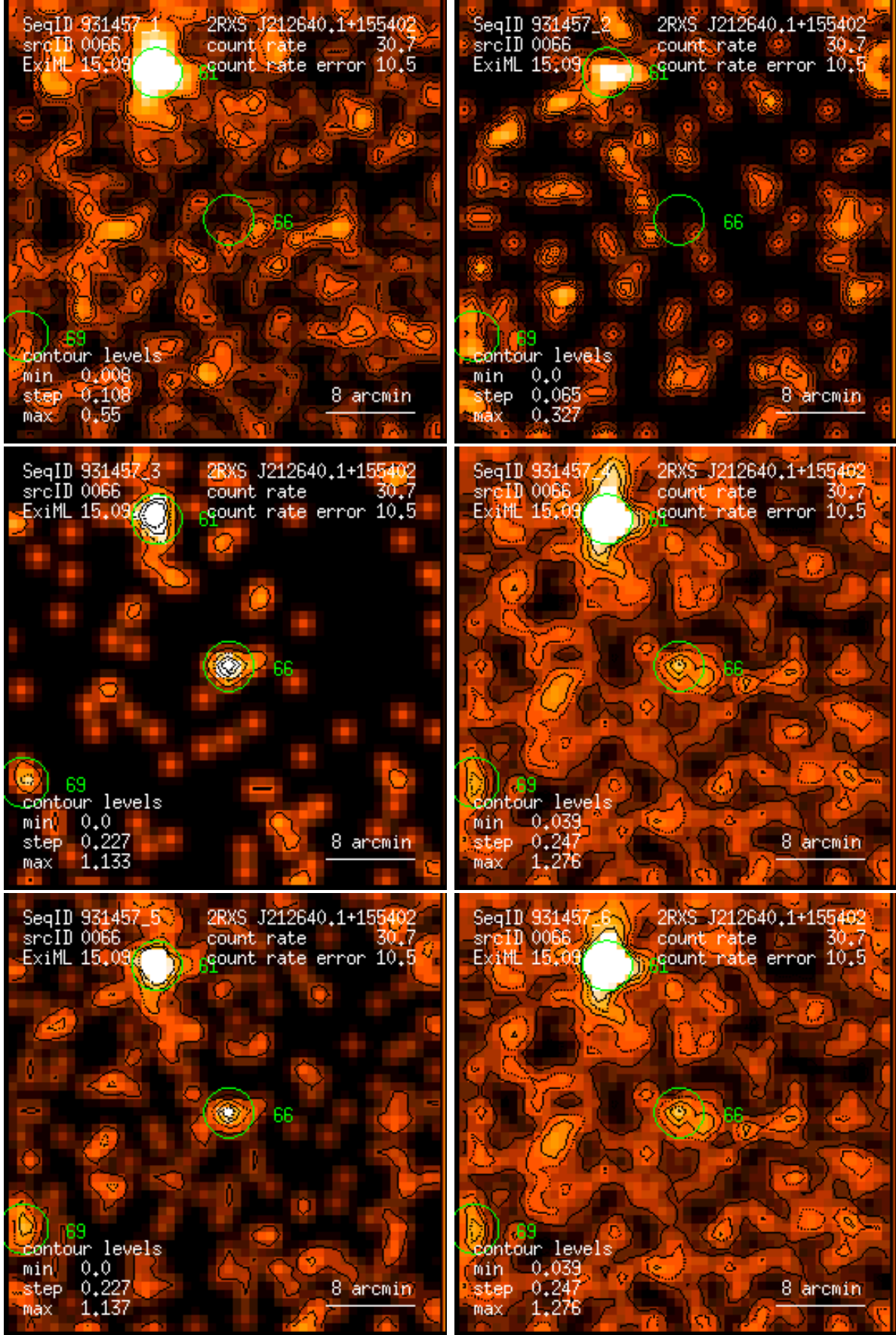
Figure 66: RASS 931457: detection 0066: band rate images, Gaussian filter: (1) PSPC channels 11 – 41, (2) 52 – 90, (3) 91 – 201, (4) 11 – 235, (5) 52 – 201, (6) 11 – 201. Broad band rates in counts/ks. Band rate contour levels in counts/ks/arcmin 2 .
