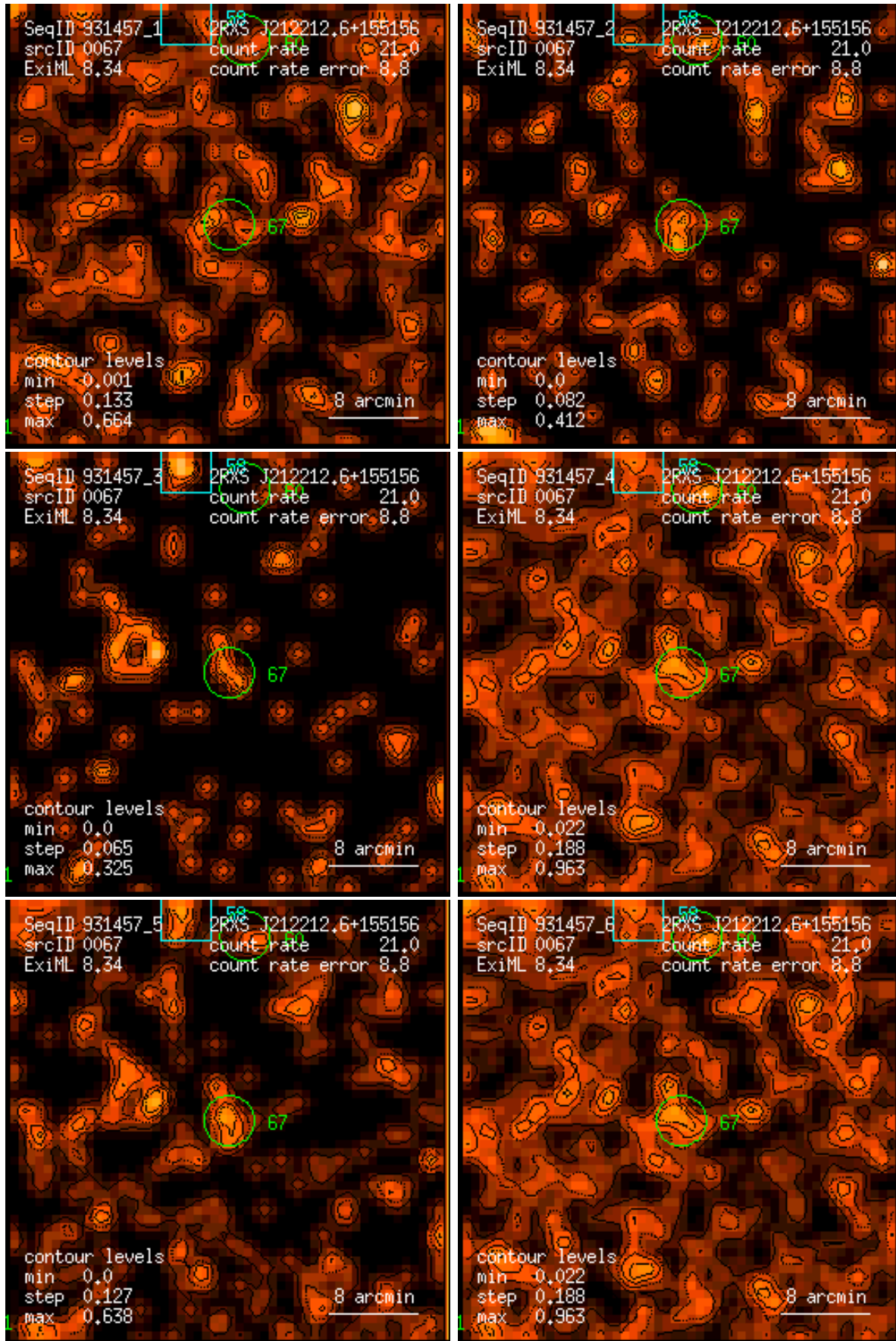
Figure 67: RASS 931457: detection 0067: band rate images, Gaussian filter: (1) PSPC channels 11 – 41, (2) 52 – 90, (3) 91 – 201, (4) 11 – 235, (5) 52 – 201, (6) 11 – 201. Broad band rates in counts/ks. Band rate contour levels in counts/ks/arcmin 2 .
