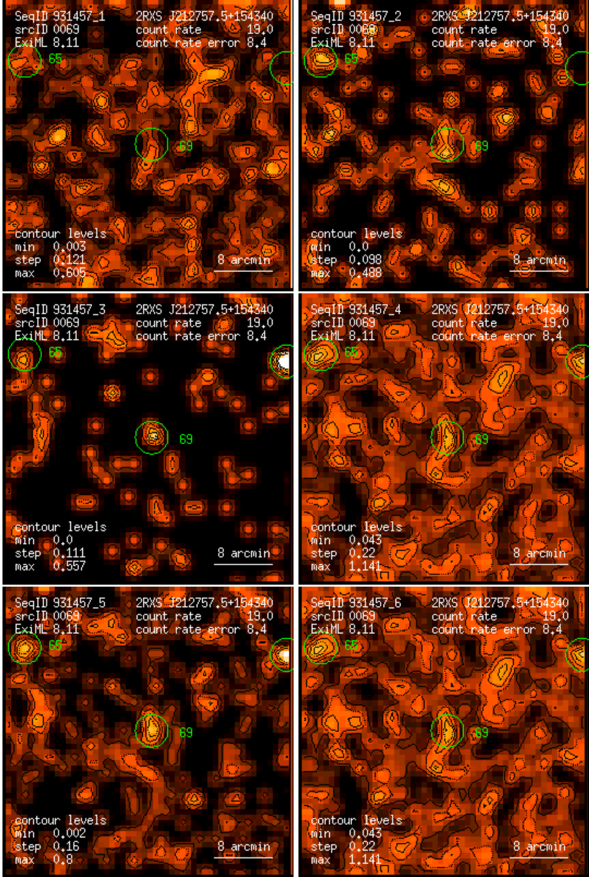
Figure 69: RASS 931457: detection 0069: band rate images, Gaussian filter: (1) PSPC channels 11 – 41, (2) 52 – 90, (3) 91 – 201, (4) 11 – 235, (5) 52 – 201, (6) 11 – 201. Broad band rates in counts/ks. Band rate contour levels in counts/ks/arcmin 2 .
